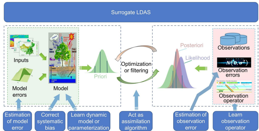
Figure 4. Integration of machine learning and LDA. Machine learning is used for model parameter optimization, model process/subprocess agent, assimilation system deviation correction, observation operator modeling, DA algorithm substitution, and LDAS surrogation.
