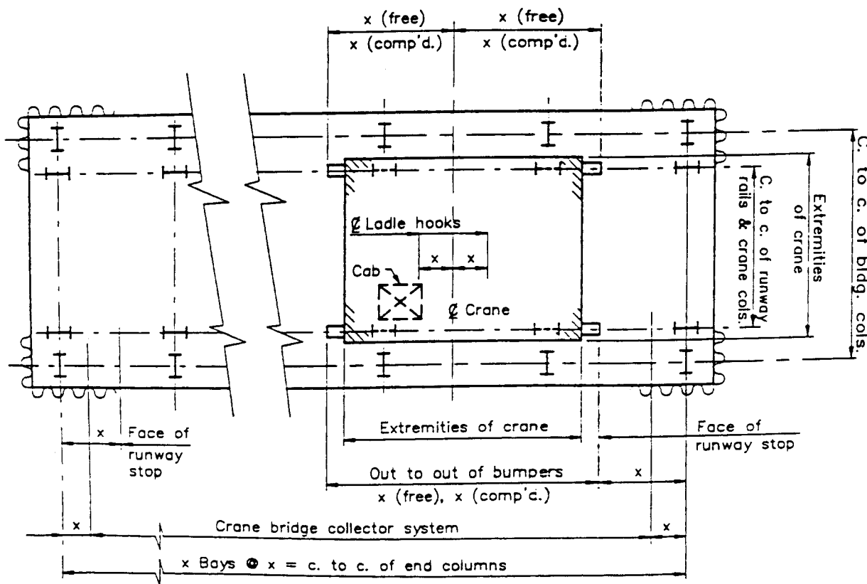
Fig. 1.2 — Plan: Typical crane runway clearance diagram.
