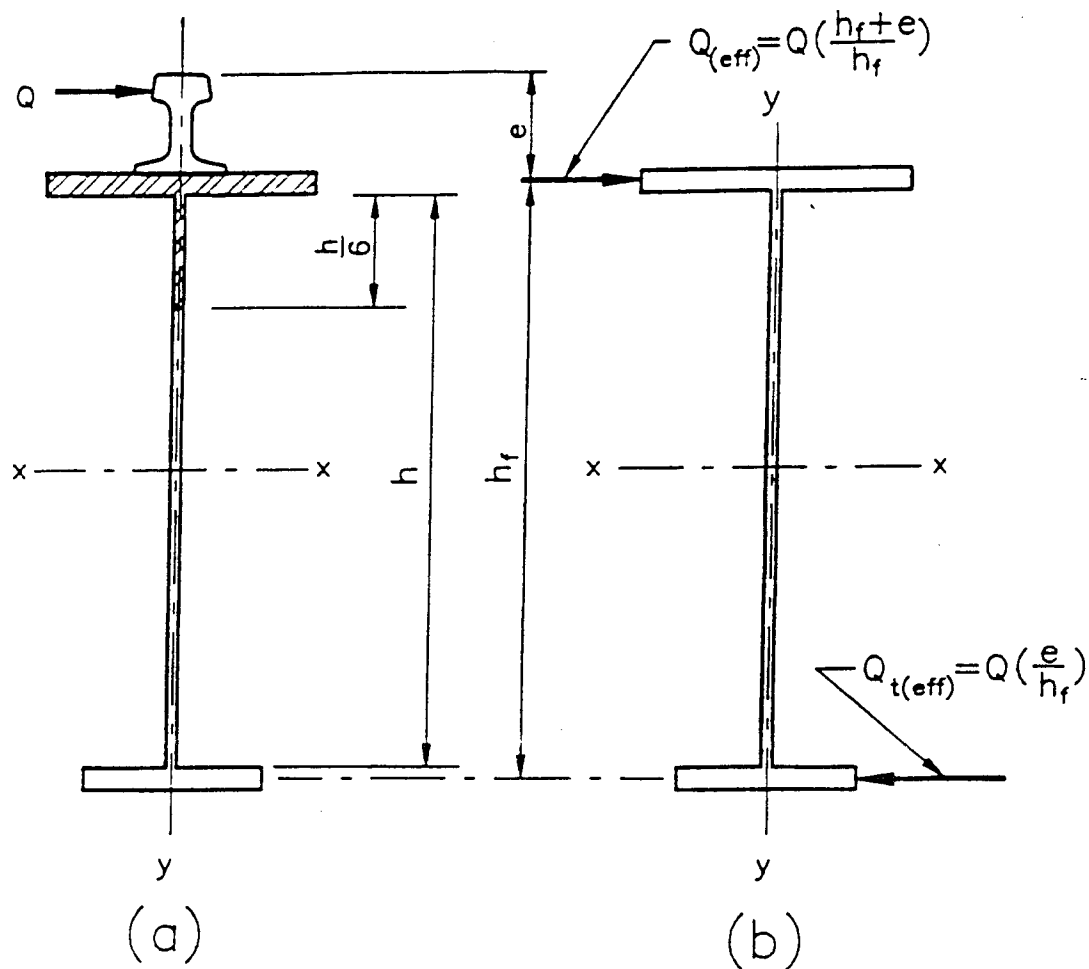
Fig. 7.3—Effective side thrust and effective area resisting side thrust in open section girders.
