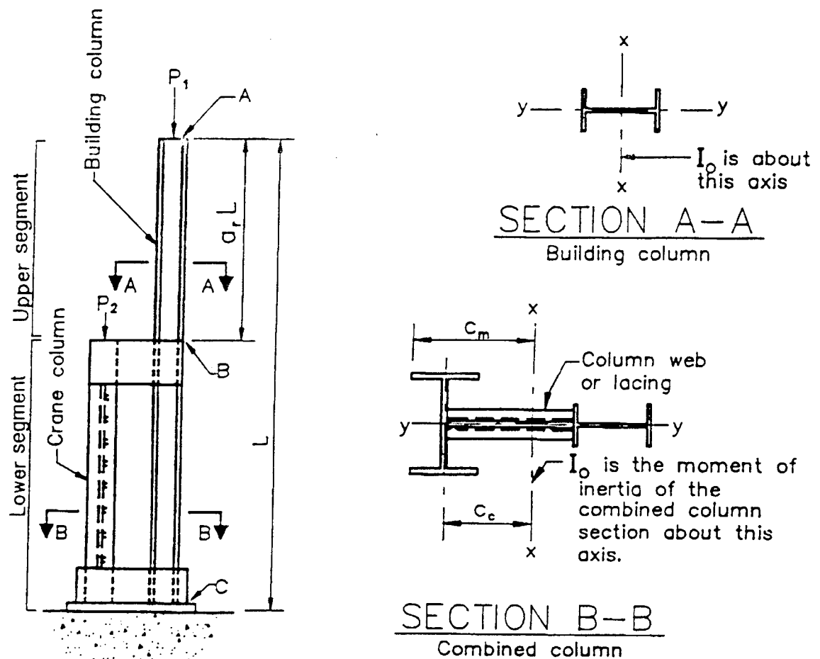
Fig. 7.4—Notation for stepped columns as used in Tables 7.1 through 7.4.
