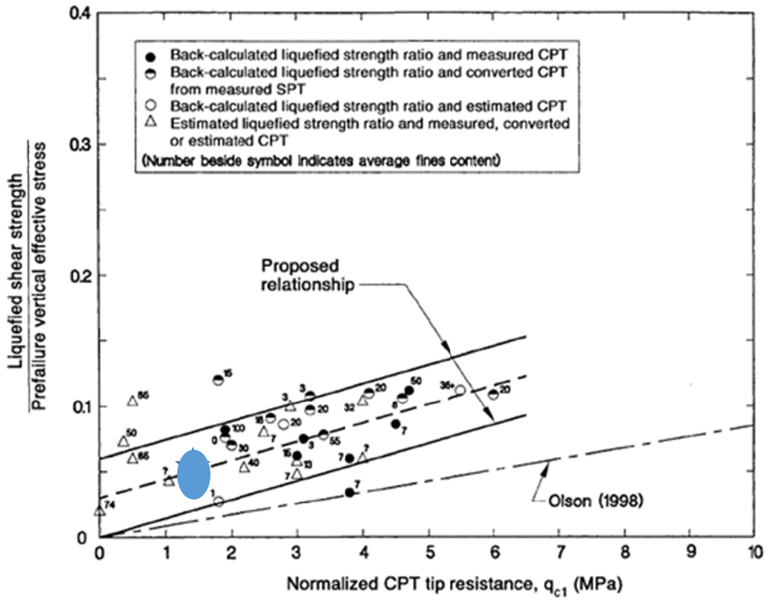
Figure 7.9 Las Palmas data point (CPT) with respect to Olson and Stark [2002].
