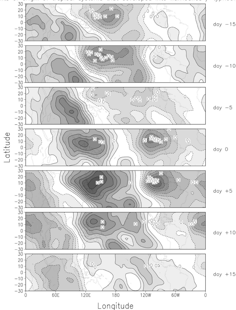
FIG. 9. Composite evolution of 200-hPa velocity potential anomalies ( 10^6 \text{ m}^2 \text{ s}^{-1} ) associated with MJO events and points of origin of tropical disturbances that developed into hurricanes or typhoons. Contour intervals are 1 \times 10^6 \text{ m}^2 \text{ s}^{-1} , solid contours indicate positive values (convection is suppressed), and dashed contours indicate negative values (convection is enhanced).
