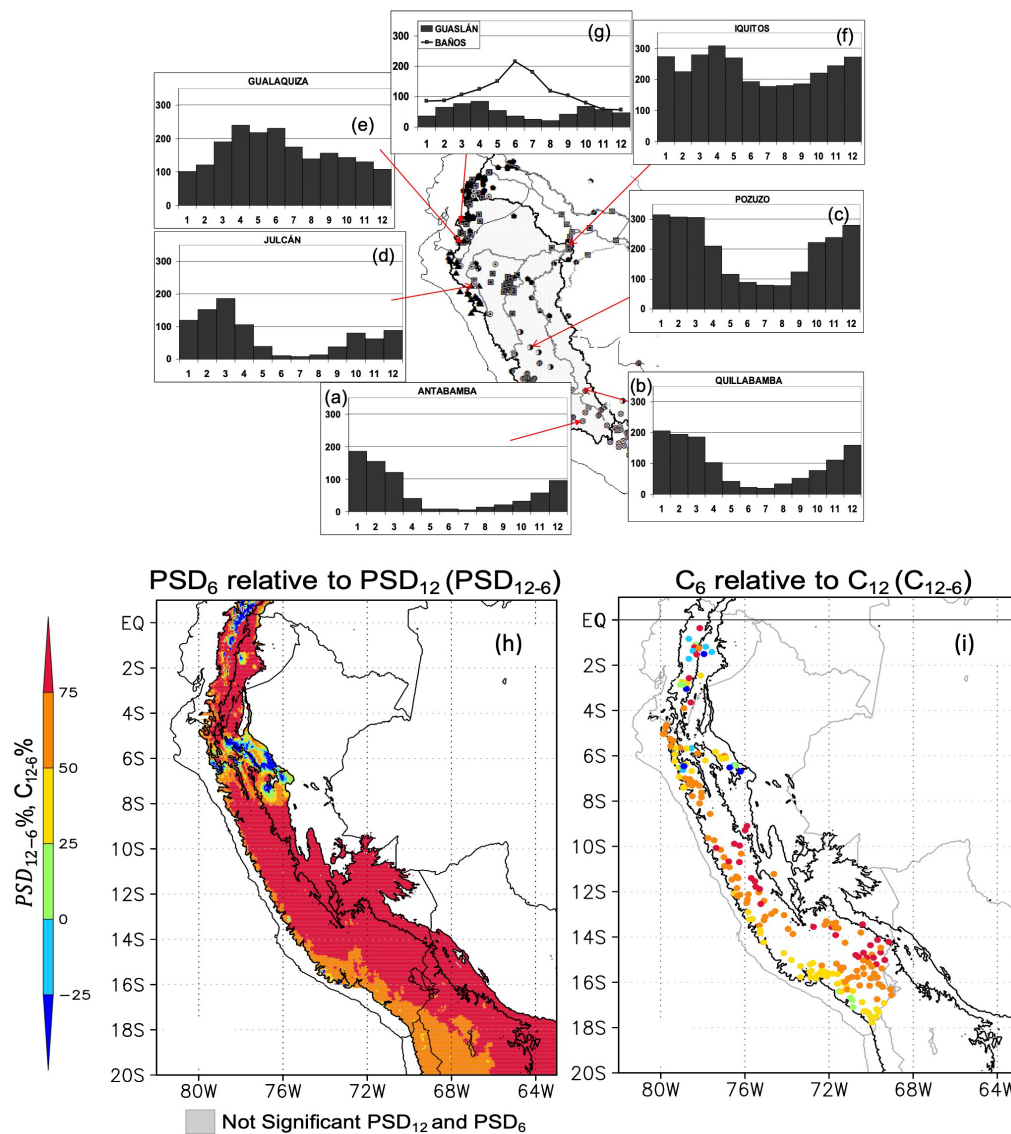
FIGURE 11 | (a–g) Rainfall regimes in eight stations in the south tropical Andes-Amazon region. Adapted from: Espinoza et al. (2009b). © International Journal of Climatology. Reprinted by permission from John Wiley and Sons. (h) Relative difference ( PSD_{12-6} ; shaded) between the maximum spectral value of monthly precipitation from 10 to 16.67 months (defined as the power spectrum density- PSD_{12} -unimodal index) and the maximum spectral value between 5 and 8 months (defined as the PSD_6 bimodal index). PSD_{12} and PSD_6 are computed using Equation 3 in Segura et al. (2019) and CHIRPS data set. (i) Relative difference between the harmonic of 12 months and the harmonic of 6 month ( C_{12-C_6} ) estimated by using in situ precipitation of 206 rain-gauge stations located in Peru and Ecuador and Equation 6 from Segura et al. (2019). Topography contours of the altitude of 350 and 2000 m.a.s.l are plotted in black solid lines. Source: Segura et al. (2019). © Climate Dynamics. Reprinted by permission from Springer Nature.
