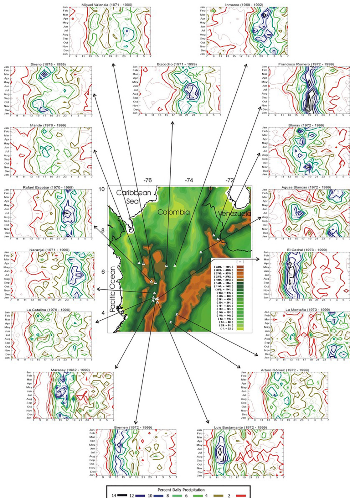
FIGURE 8 | Seasonal march of the diurnal cycle of rainfall at 17 selected stations in the north tropical Andes of Colombia (north of 8°S). The diurnal cycle is defined from 0700 to 0700 local standard time (LST), and interpolated isolines indicate percent of total daily rainfall, with the color scale shown at the bottom. Boundaries of the neighboring (left) Cauca and (right) Magdalena River valleys are shown in white. The inset at the bottom left shows details of rain gauges located in the western flank of the central range of the Colombian Andes. Source: Poveda et al. (2005). © American Meteorological Society. Used with permission.
