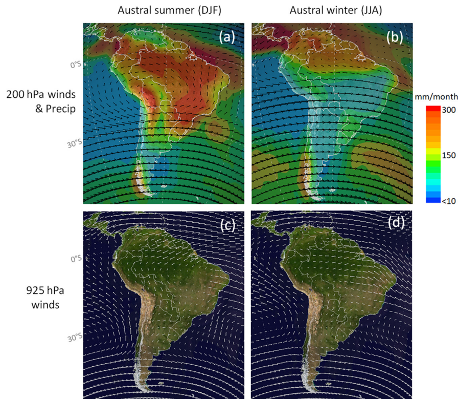
FIGURE 1 | (a,b) Long-term mean (1981–2020) winds at 200 hPa (arrows) and precipitation (shades). (c,d) Long-term mean (1981–2020) winds at 925 hPa (arrows) over blue marble. Data from NCEP/NCAR reanalysis.
