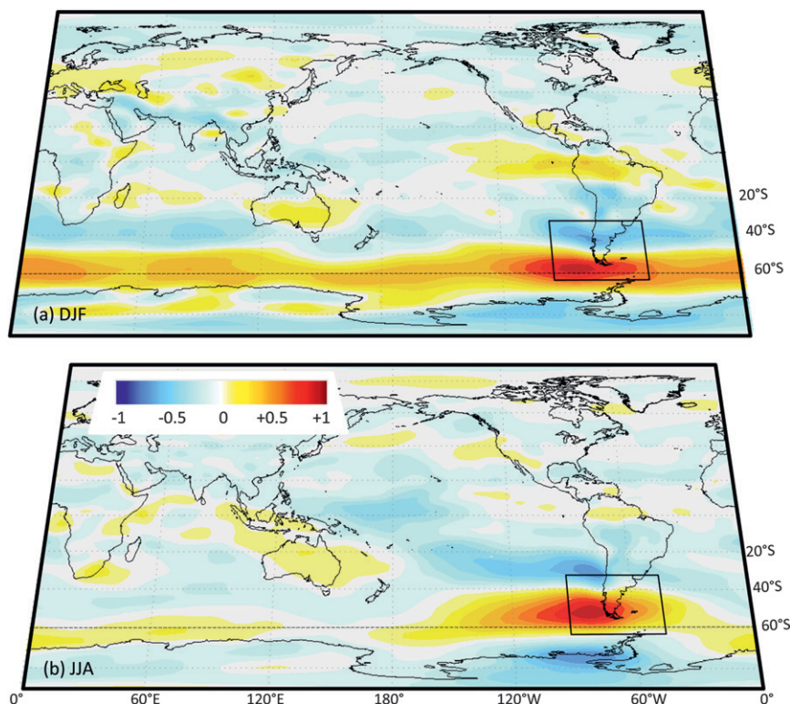
FIG. 9. Leading mode of the 850-hPa zonal ( U_{850} ) wind interannual variability over southern South America and the adjacent oceans in austral (a) summer and (b) winter using NCEP–NCAR reanalysis data. The EOF analysis was performed for each month in the area outlined by the solid rectangle ( 35^{\circ} – 65^{\circ} S, 90^{\circ} – 60^{\circ} W) and the resulting principal component (time series) was projected on the global U_{850} field. The summer (winter) map was constructed by averaging the DJF (JJA) values at each grid box.
