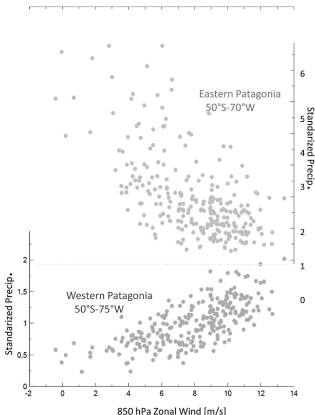
FIG. 6. Scatterplot between monthly precipitation and 850-hPa zonal wind in western and eastern Patagonia. Here we used PRECIS-DGF values from 1978–2001 in two 2^\circ \times 2^\circ boxes centered at 50^\circ\text{S} , 75^\circ\text{W} and 50^\circ\text{S} , 70^\circ\text{W} . The precipitation values were standardized dividing by their respective long-term means.
