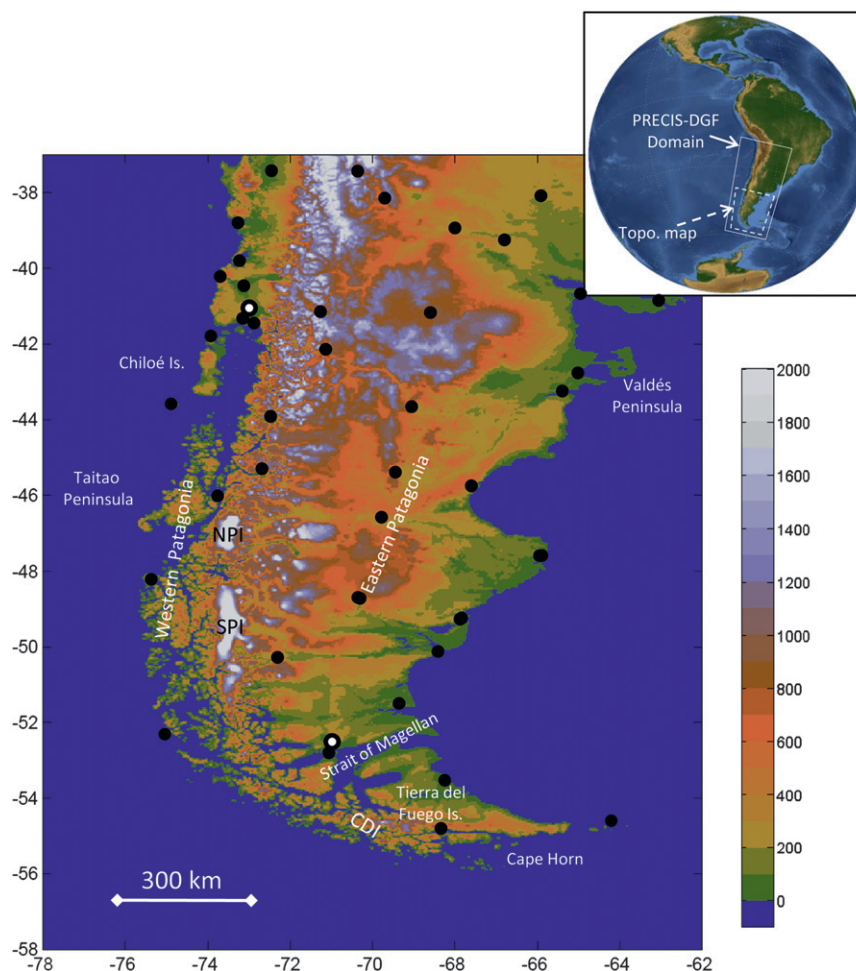
FIG. 1. Topographic map of southern South America (color scale in m MSL) highlighting key features in the Patagonia region. Black circles indicate the location of the meteorological stations used in this work (precipitation and surface air temperature). White circles indicate the location of the regular upper-air (radiosonde) stations: Puerto Montt and Punta Arenas. The upper inset shows the PRECIS-DGF domain used in this work.
