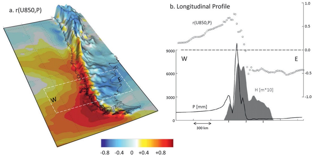
FIG. 5. (a) Local (point to point) correlation between annual mean 850-hPa zonal wind and precipitation [ r(U_{850}, P) ] using PRECIS-DGF results from 1978 to 2001. For display purposes the correlation values are shown over the model topography. (b) Longitudinal profile of terrain elevation (shaded area, scale at left), long-term-mean annual precipitation (black line, scale at left in mm \text{ yr}^{-1} ), and the r(U_{850}, P) correlation, averaged between 42^\circ and 52^\circ\text{S} . The profiles were constructed every 0.5^\circ of latitude and then composited taken the longitude of highest elevation as a horizontal reference.
