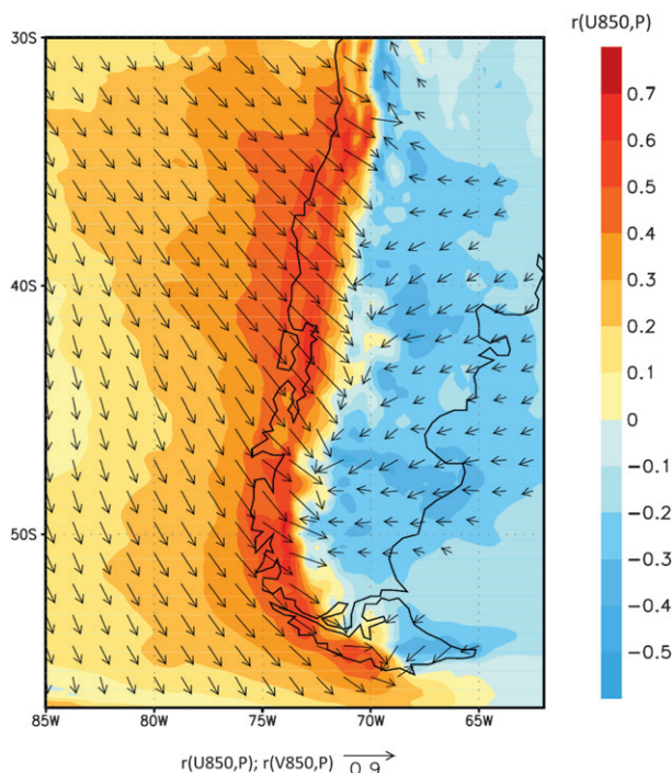
FIG. 4. Local (point-to-point) correlation map between daily precipitation ( P ) and 850-hPa zonal and meridional wind components ( U_{850} ; V_{850} ) using PRECIS-DGF results from 1980–90. At each grid point the correlation was calculated for the sample of days with P > 1 mm. Colors indicate the P – U_{850} correlation. Vectors are constructed using r(P, U_{850}) and r(P, V_{850}) (scale at the bottom) and only shown where absolute value exceeds 0.3.
