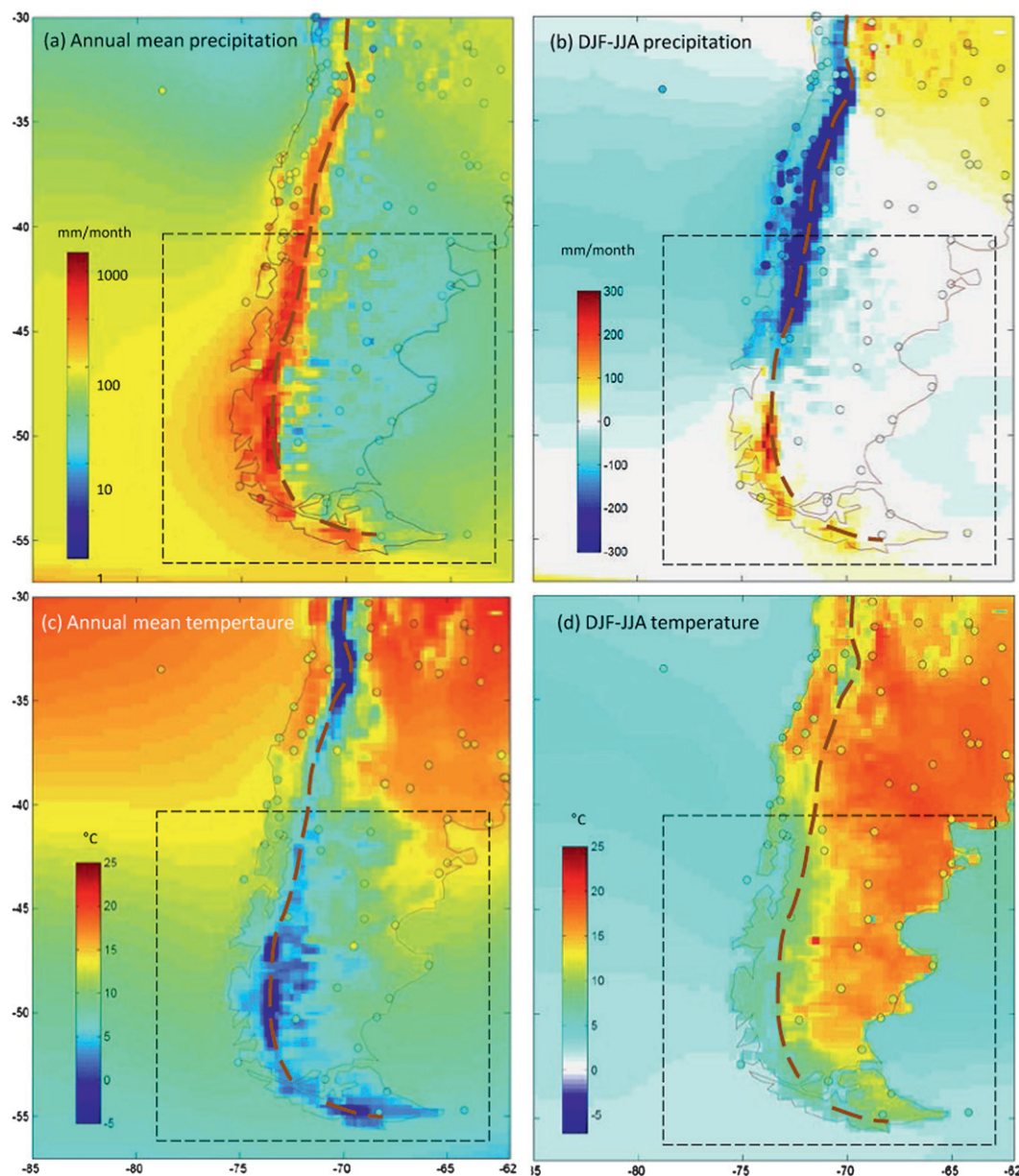
FIG. 2. Comparison of the PRECIS-DGF climatology (shaded) against station observations (circles filled with the same color scale). The model climatology is computed using the period 1978–2001; the station climatology is calculated using all available monthly data during the second half of the twentieth century. Dashed line indicates the ridge of the Andes. (a) Annual mean precipitation; note the logarithmic color scale. (b) Austral summer (DJF) minus winter [June–August (JJA)] mean precipitation. (c) Annual mean near-surface air temperature (1.5 m in the model; approximately 2 m in observations). (d) Austral summer (DJF) minus winter (JJA) mean near-surface air temperature.
