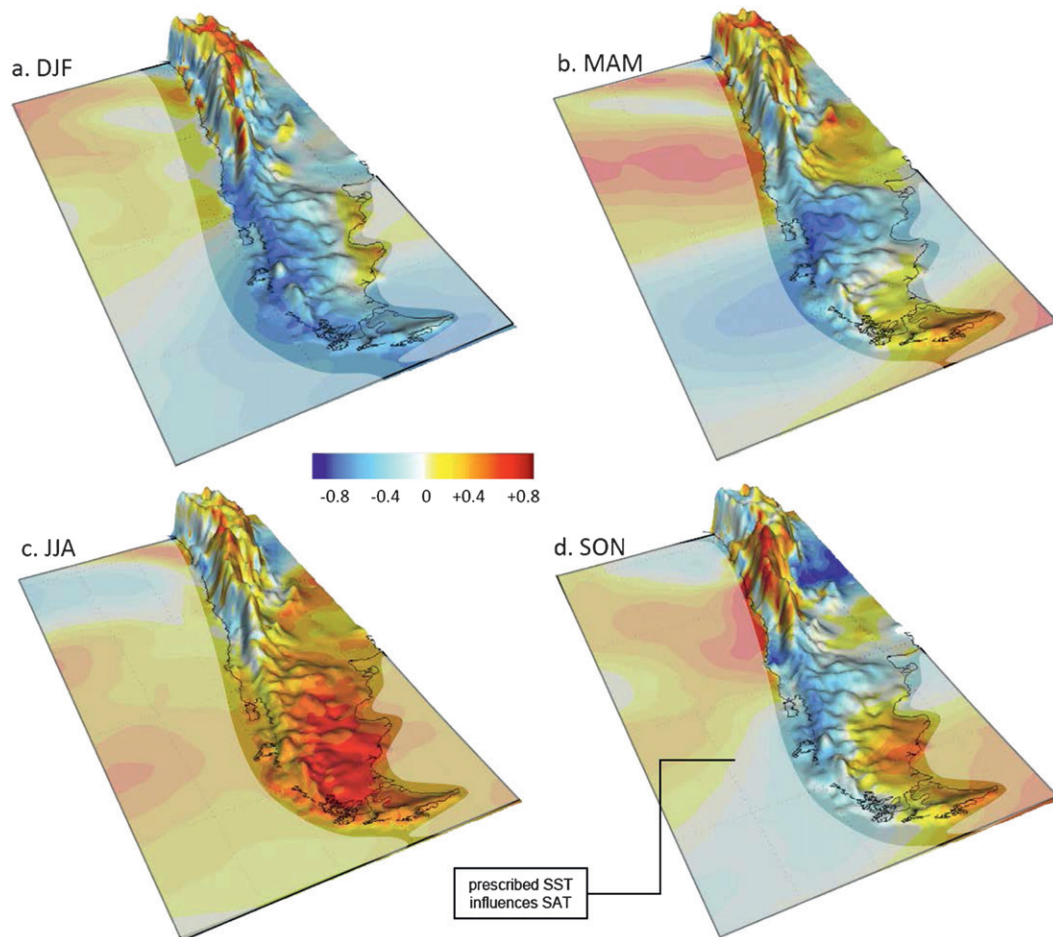
FIG. 8. Local (point to point) correlation between seasonal mean 850-hPa zonal wind and surface air temperature, using PRECIS-DGF results from 1978 to 2001. For display purposes the correlation values are displayed over a 3D topography. The r(U_{850}, SAT) values over ocean are slightly masked since SAT there is strongly controlled by the sea surface temperature, which is prescribed in PRECIS-DGF.
