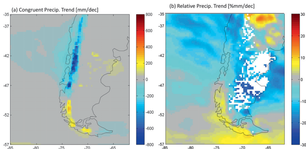
FIG. 12. Annual mean precipitation changes in the period 1968–2001 congruent with the reanalysis (NNR and ERA-40) zonal wind changes (see text for details). (a) Absolute changes in \text{mm decade}^{-1} . (b) Absolute changes ( \text{mm decade}^{-1} ) standardized by the long-term-mean annual precipitation (derived from PRECIS-DGF). The relative changes are not shown in areas where the annual mean precipitation is less than 300 \text{ mm yr}^{-1} .
