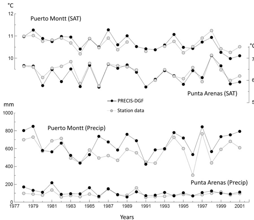
FIG. 3. Time series of observed (gray circles) and PRECIS-DGF (black circles) annual mean near-surface (top) air temperature and (bottom) precipitation in Puerto Montt (northwestern Patagonia; 41.5°S, 72.8°W) and Punta Arenas (southeastern Patagonia; 53.2°S, 70.9°W).
