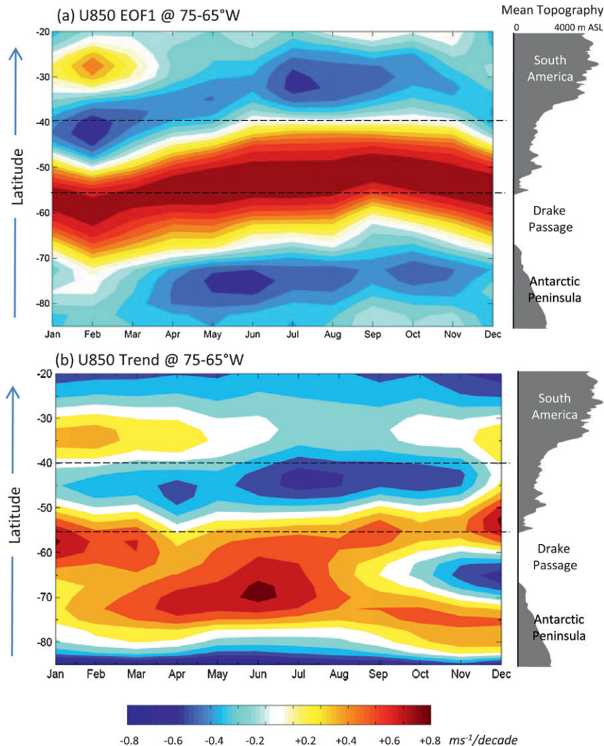
FIG. 10. (a) Latitudinal–seasonal variation of the leading mode of the 850-hPa zonal wind ( U_{850} ) interannual variability averaged between 75° and 65°W. The EOF analysis was performed for each month in the area outlined in Fig. 10. (b) Linear trends (1968–2001) in U_{850} averaged between 75° and 65°W. The gray area to the right shows the mean topography. Results are based on NCEP–NCAR reanalysis.
