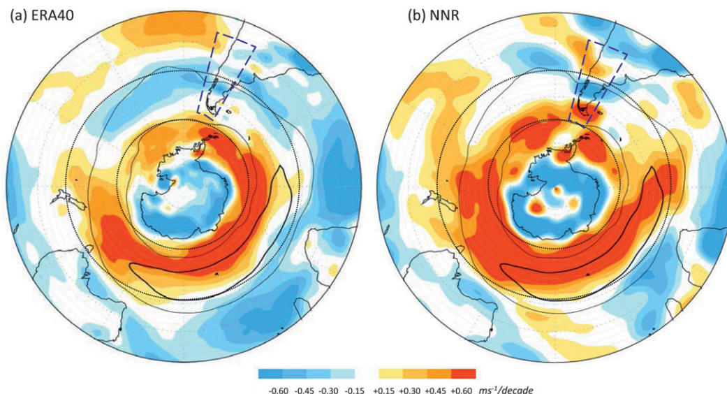
FIG. 11. Linear trends in the annual mean zonal wind at 850 hPa ( U_{850} ) using the (a) ERA-40 and (b) NCEP–NCAR reanalyses. Shading indicates the change between 1968 and 2001 of a linear least squares trend fit calculated at each grid box. The thick (thin) black contour outlined areas where the annual mean U_{850} exceeds 15 \text{ m s}^{-1} ( 10 \text{ m s}^{-1} ).
