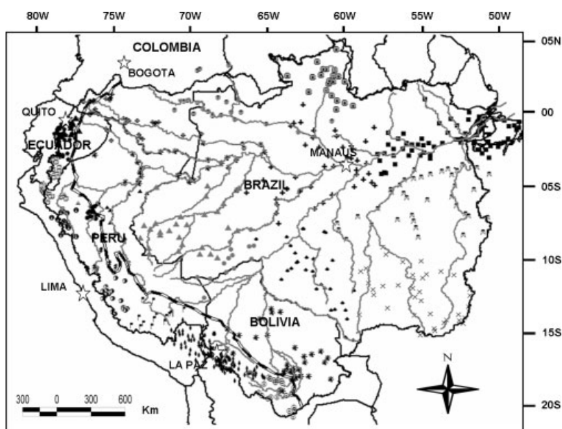
Figure 1. Limit of the Amazon basin (solid line) and of the Andean regions above 500 m (black and white line) and location of the rainfall gauges approved by the regional vector method (756 stations with more than 5-year records). The 25 symbols represent the groups of stations from which the 25 vectors were created.
