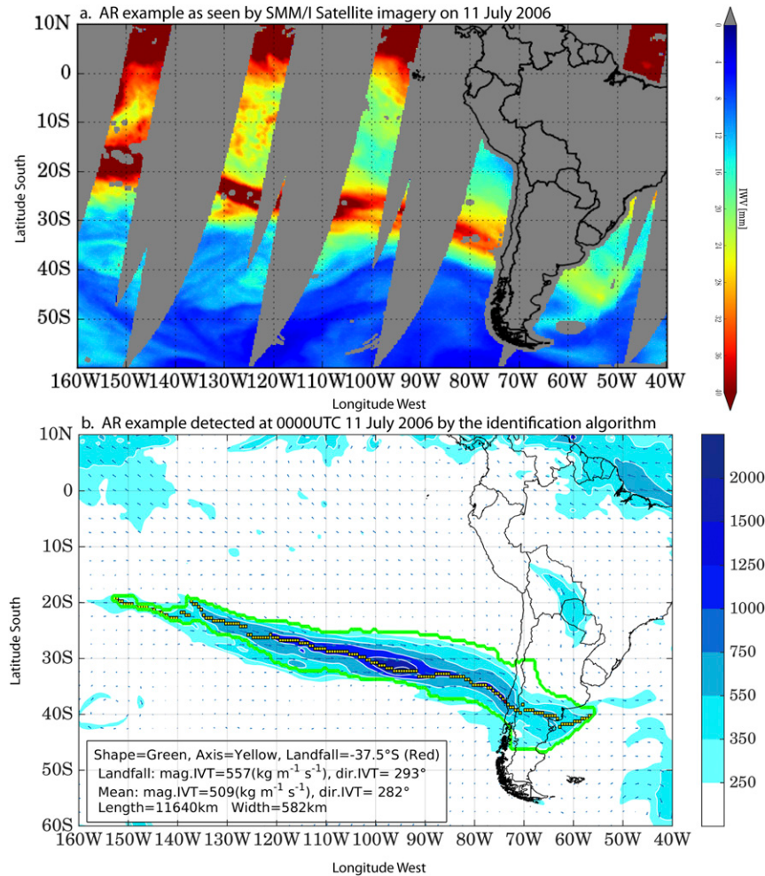
FIG. 3. (a) Chart of the IWV (mm) as seen by the SMM/I satellite imagery during the morning passes on 11 Jul 2006 showing an AR example. (b) Chart of the IVT ( \text{kg m}^{-1} \text{s}^{-1} ) magnitude and direction (color shading and vectors, respectively) showing the AR example detected at 0000 UTC 11 Jul 2006 by the algorithm. The algorithm outputs of the shape boundary (green), axis (yellow), landfall location (red), and other key metrics are shown in the bottom-left corner. This case was one of the most devastating ARs over the period of 2001–16.
