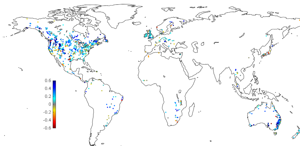
Figure 5. For the evaluation catchments, the AOF score obtained by HBV with regionalized parameters based on the 10 most similar donors minus the AOF score obtained using the spatially uniform parameters (defined as AOF change). Blue indicates enhanced model performance using regionalized parameters while yellow and red indicate diminished model performance using regionalized parameters. Each data point represents a catchment centroid ( n = 1113 ). HBV was driven by CPC precipitation.
