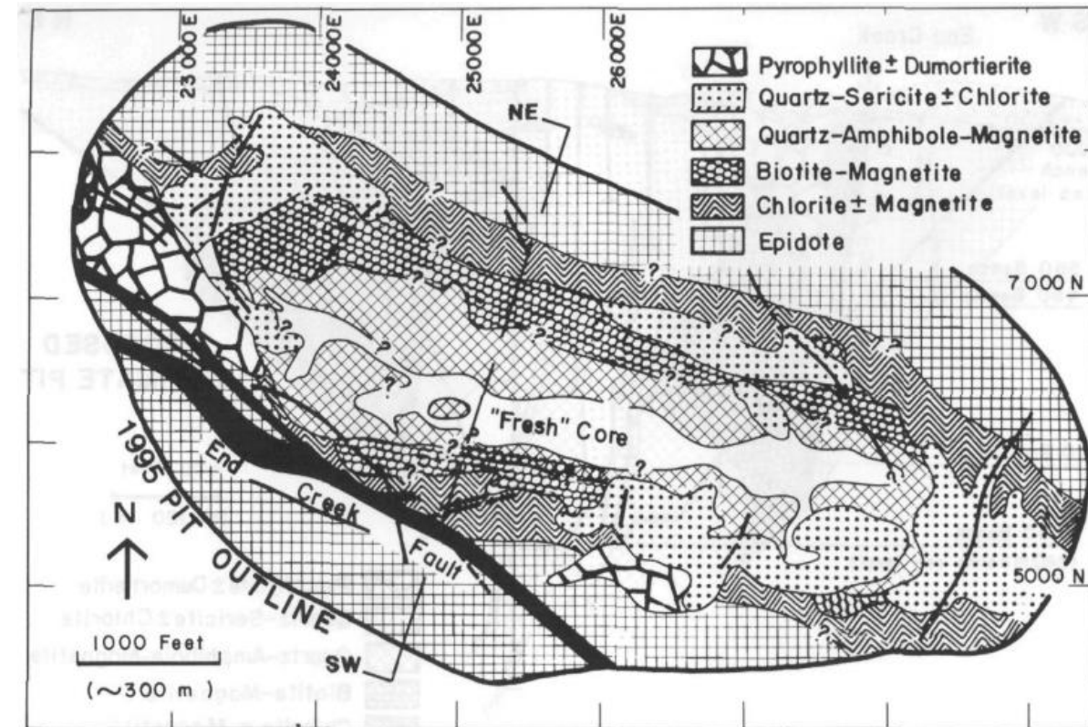
Geology at BHP Island Copper mine
