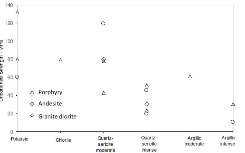
Relationship between the uniaxial compressive strength of intact rock and the type of alteration, based on Chuquicamata samples (Hoek et al. 2000)
