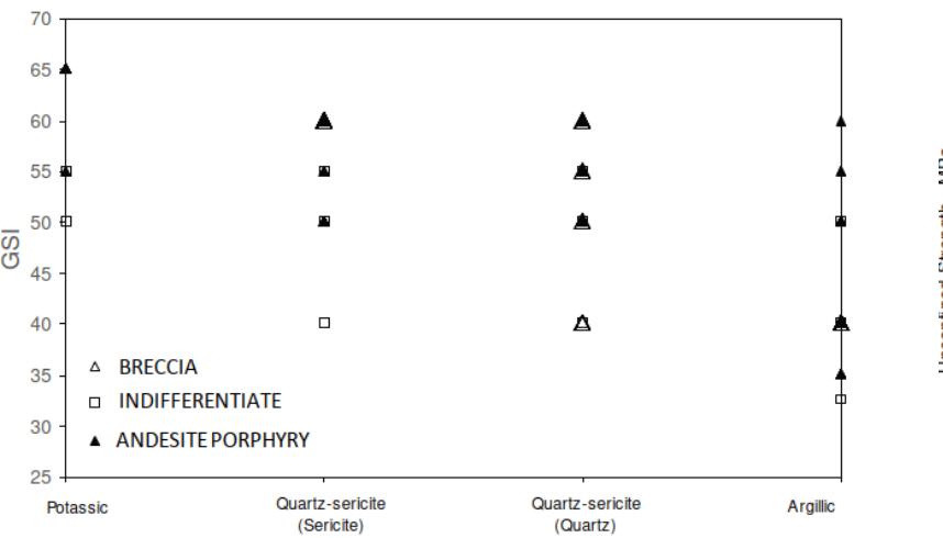
4 Relationship between Geological Strength Index (GSI) and grades of alteration based on 1,775 mapped samples from BHP sites in Chile. A decreasing trend of GSI values is observed from potassic to argillic alteration
