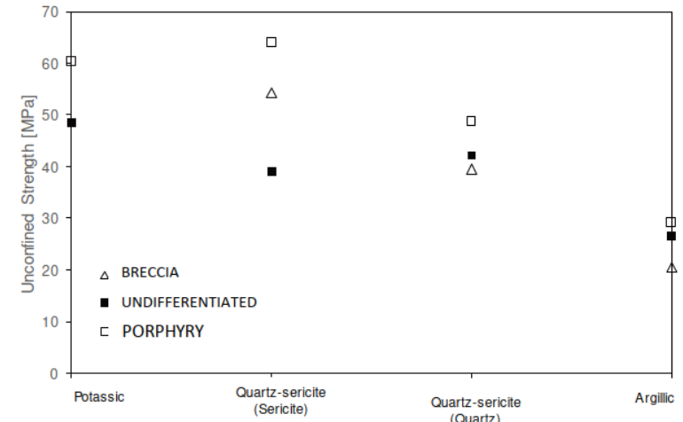
Relationship between the uniaxial compressive strength of intact rock and the type of alteration for different types of rock. Average values based on 1,775 samples from BHP sites in Chile
