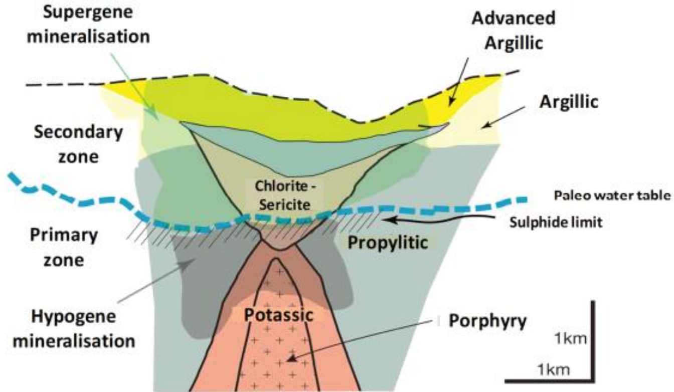
Generalised scheme of sequence of alteration-mineralisation of porphyry copper systems, indicating the secondary-primary limit, usually associated to the limit of sulphide presence (modified from Sillitoe 2010)
