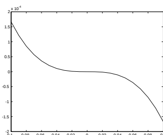
o(x) = \sin(x) - x
