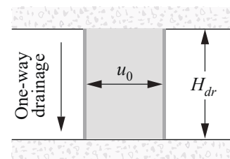
Different types of drainage with u_0 constant
