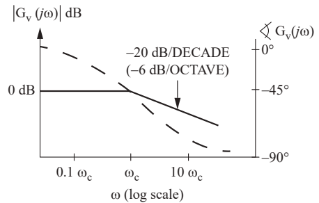
(e) (1 + j\omega/\omega_c)^{-1}
