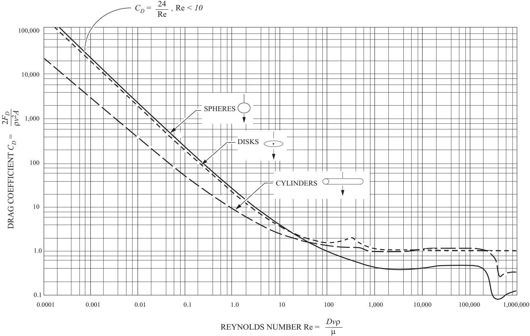
Drag Coefficient for Spheres, Disks, and Cylinders
