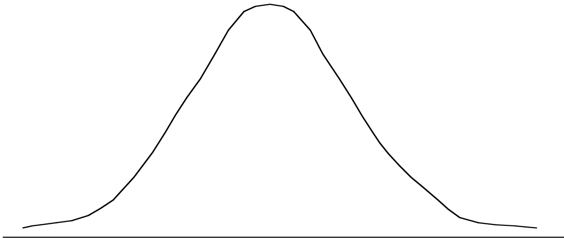
Figure 1: Normal Distribution
