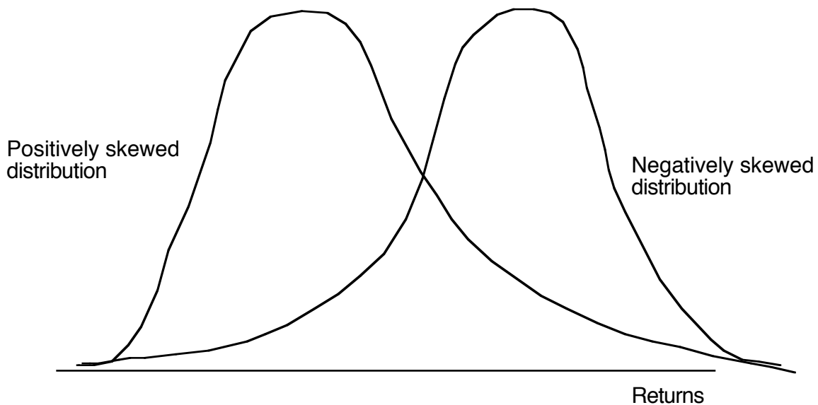
Figure 2: Skewed Distributions
