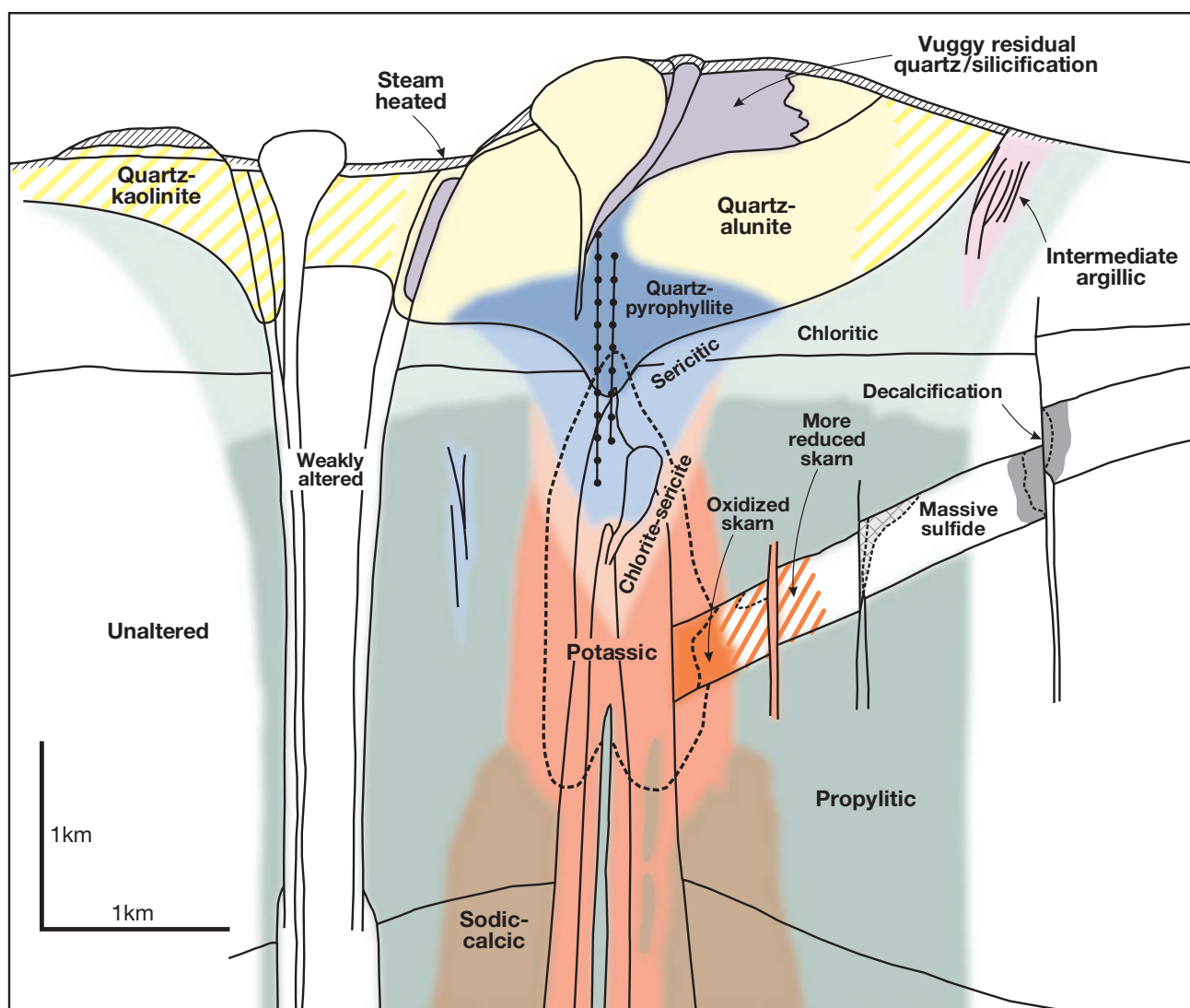
FIG. 10. Generalized alteration-mineralization zoning pattern for telescoped porphyry Cu deposits, based on the geologic and deposit-type template presented as Figure 6. Note that shallow alteration-mineralization types consistently overprint deeper ones. Volumes of the different alteration types vary markedly from deposit to deposit. Sericitic alteration may project vertically downward as an annulus separating the potassic and propylitic zones as well as cutting the potassic zone centrally as shown. Sericitic alteration tends to be more abundant in porphyry Cu-Mo deposits, whereas chlorite-sericite alteration develops preferentially in porphyry Cu-Au deposits. Alteration-mineralization in the lithocap is commonly far more complex than shown, particularly where structural control is paramount. See text for further details and Table 2 for alteration-mineralization details. Modified from Sillitoe (1999b, 2000).
