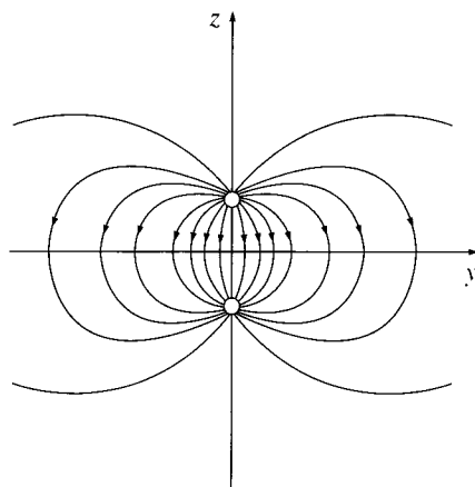
(a) Field of a “physical” dipole
