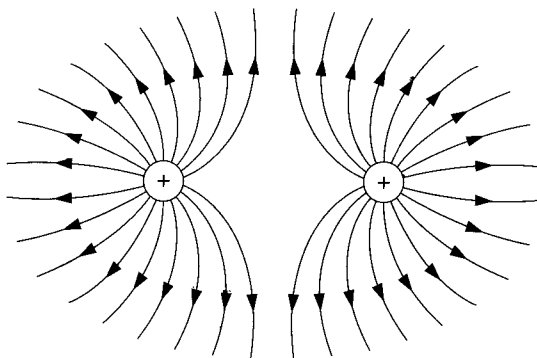
Equal charges
