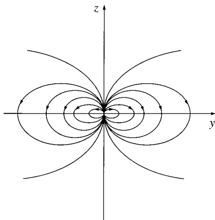
(a) Field of a “pure” dipole
