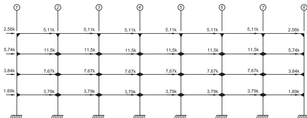
FRAME (1/2 BLDG)
