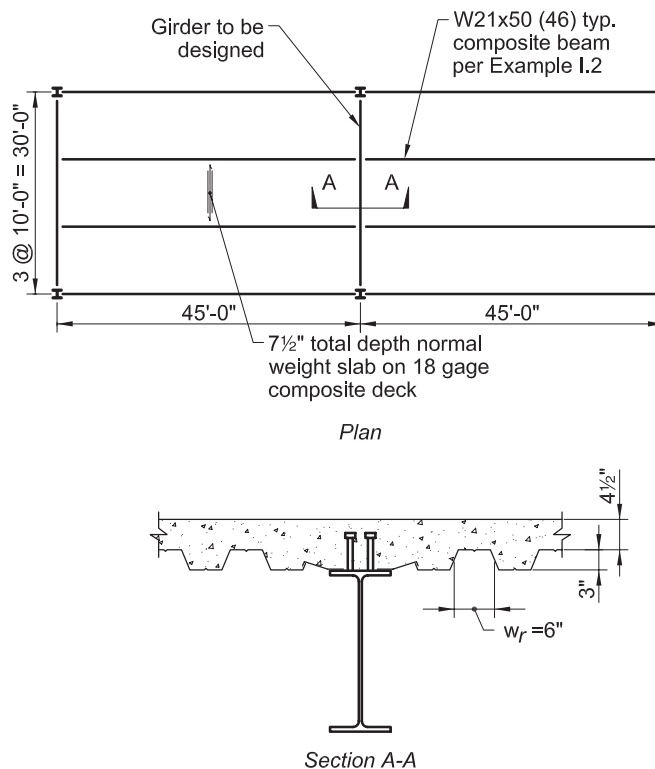
Fig. I.2-1. Composite bay and girder section.
