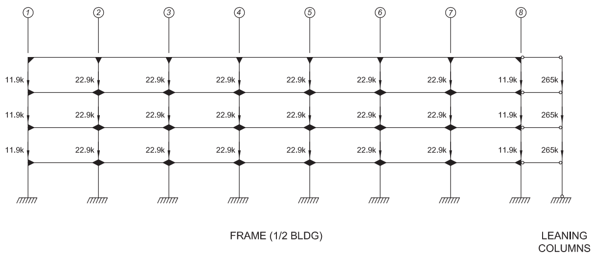
NOMINAL LIVE LOADS
