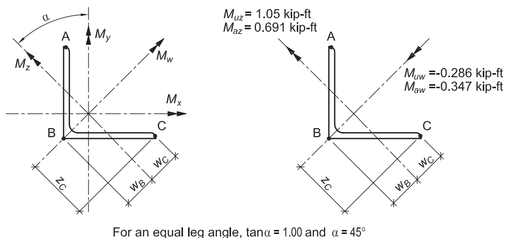
Positive Geometric and Principal Axes
