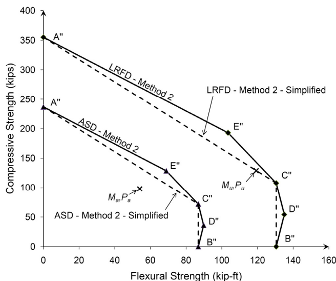
Fig. I.6-6. Comparison of Method 2 and Method 2 – Simplified.
