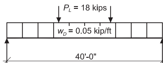
Beam Loading & Bracing Diagram (continuous bracing)
