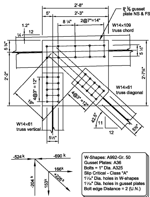
Example Connection Using Bolted Gusset Plates @ Top Chord Panel Point U3 of Example Truss Design Case 2: ASD Design Format
