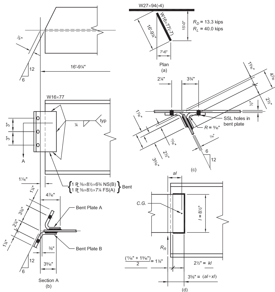
Fig. IIA-10. Skewed Double Bent-Plate Connection (Beam-to-Girder Web)
