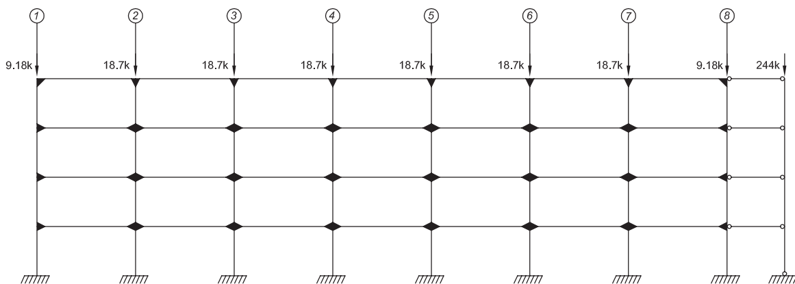
FRAME (1/2 BLDG)
