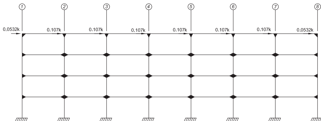
FRAME (1/2 BLDG)
