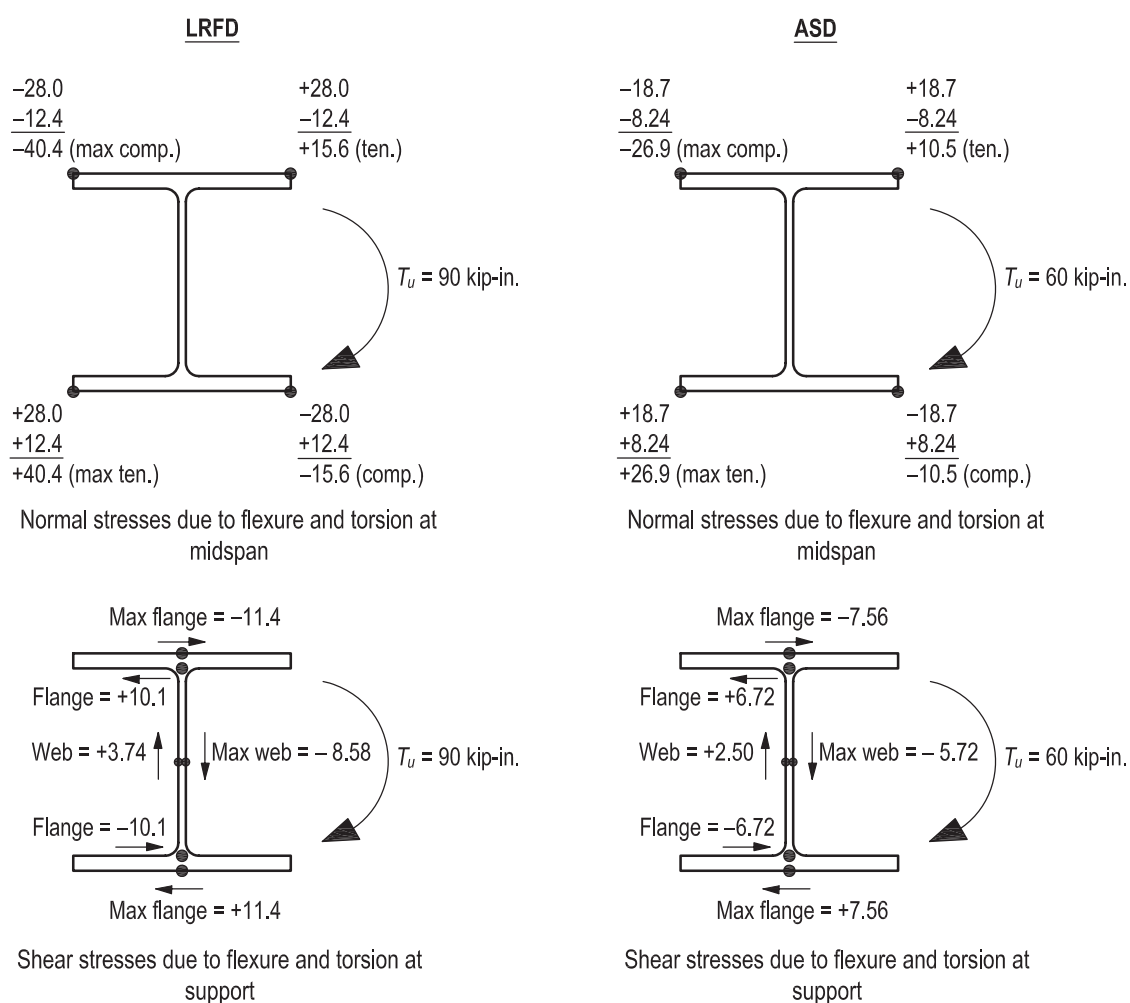
Fig. H.6-1. Stresses due to flexure and torsion.
