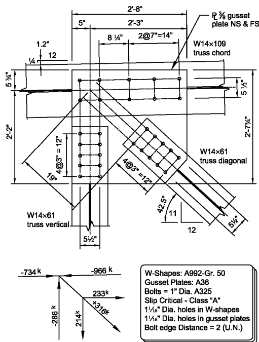
Example Connection Using Bolted Gusset Plates @ Top Chord Panel Point U3 of Example Truss Design Case 1: LRFD Design Format
