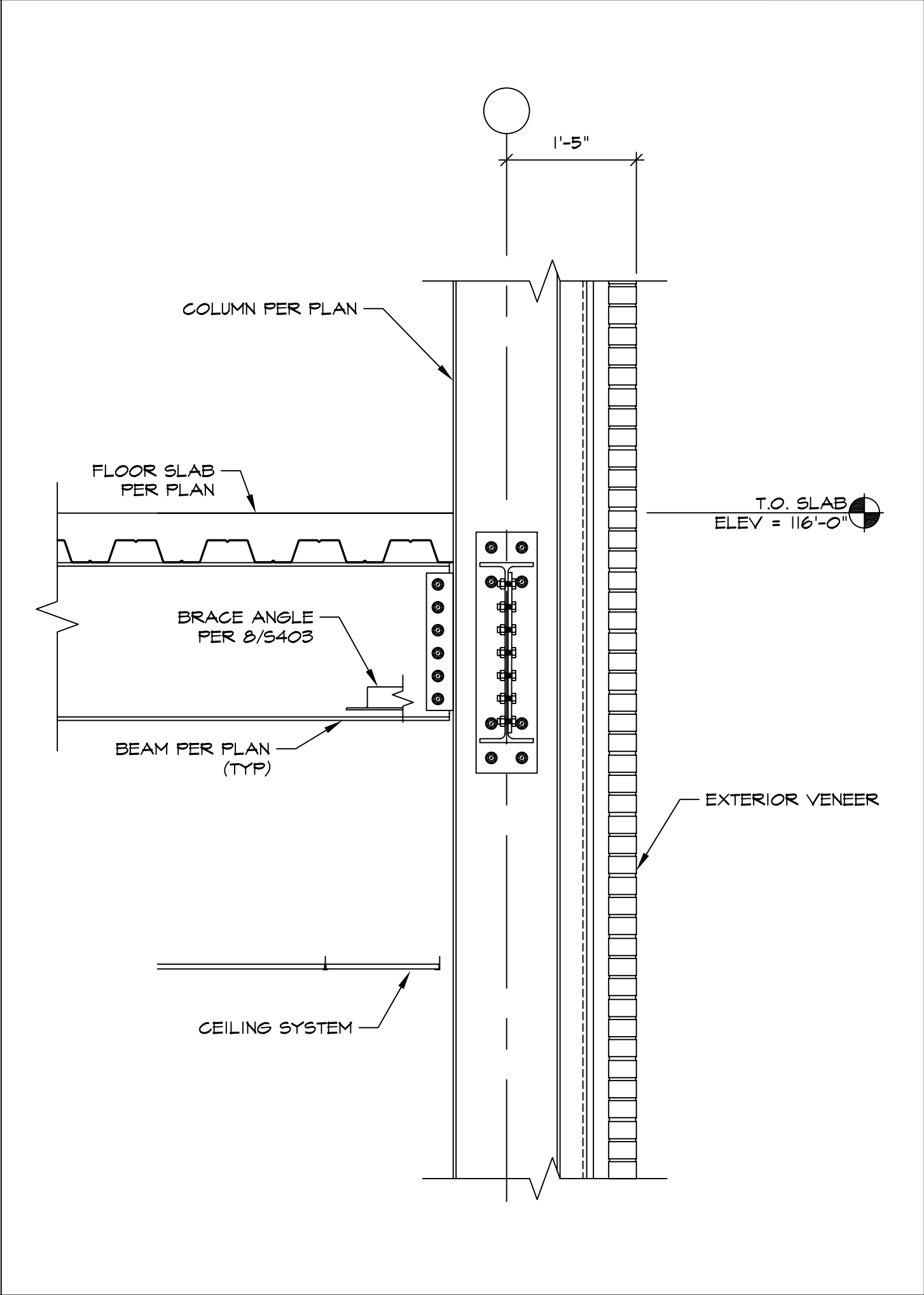
SECTION 3/4" = 1'-0"
