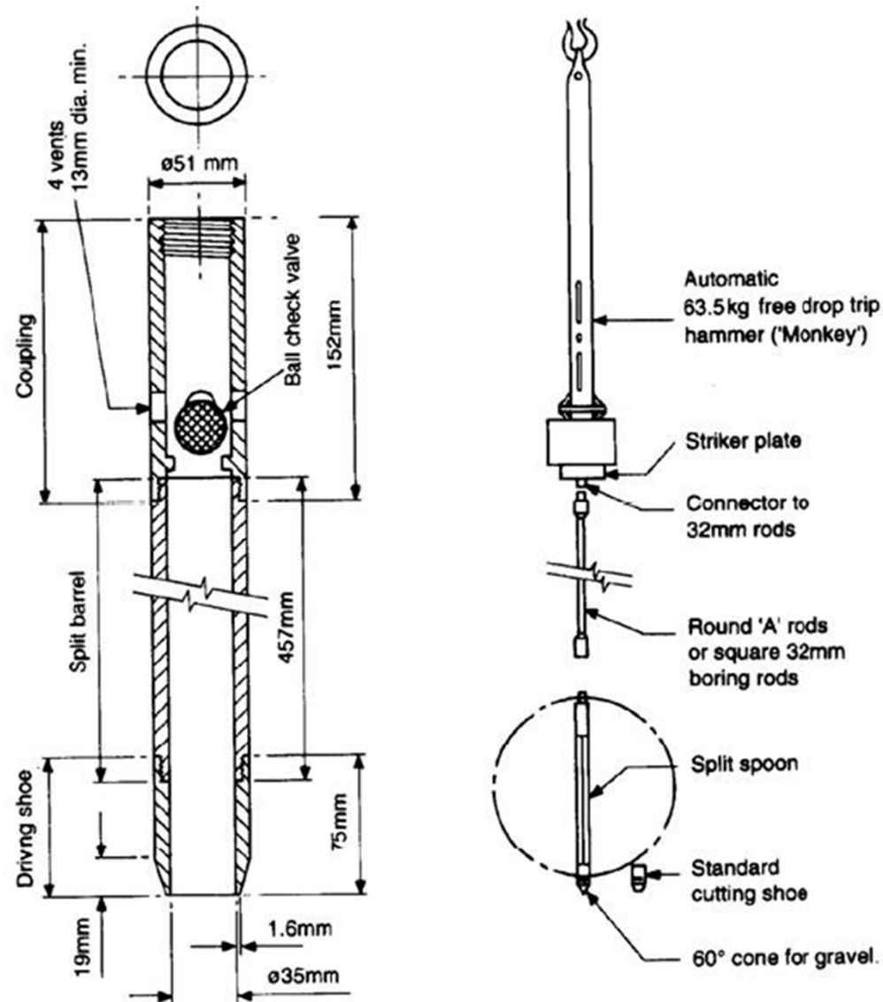
Fig. 9.1 Equipment for the standard penetration test.
