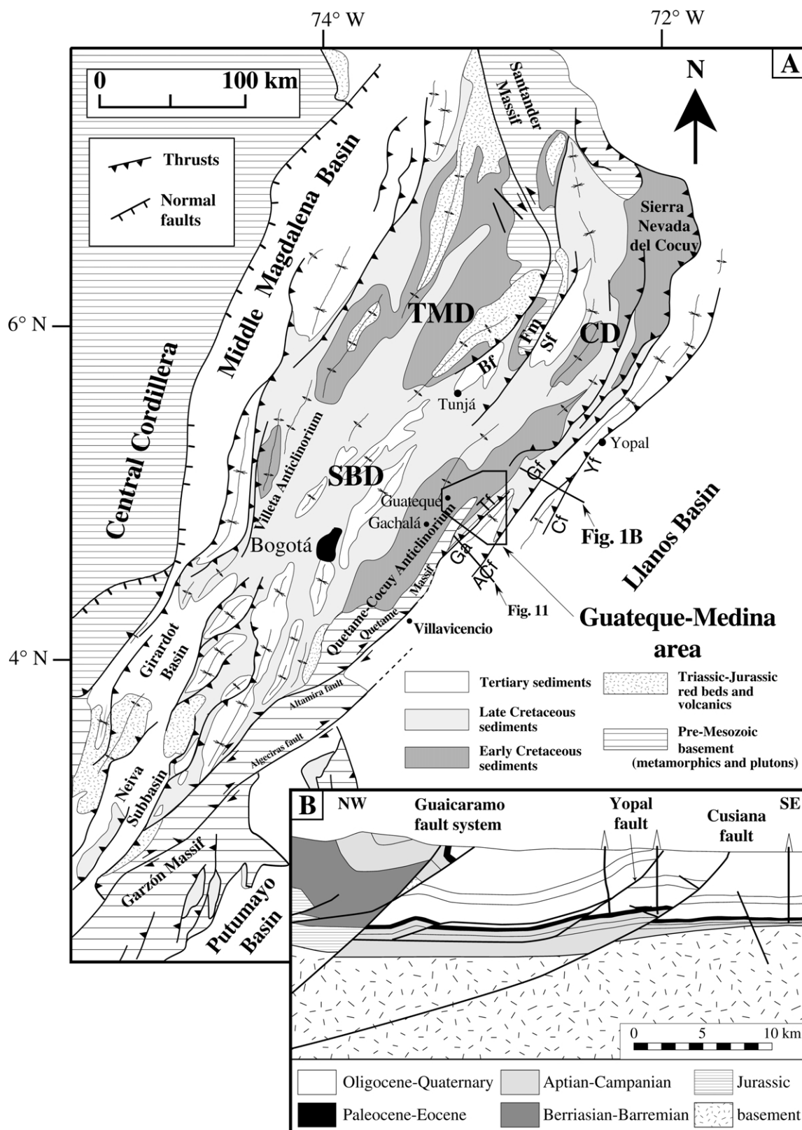
Fig. 1. (A) Structural map of the Cordillera Oriental (modified from Schamel (1991) and González et al. (1988)). Early Cretaceous depocenters (TMD: Tablazo–Magdalena; CD: Cocuy) merge southward into single Sabana de Bogotá depocenter (SBD). Ga: Guavio anticline; ACf: Agua Clara fault, Gf: Guaicáramo fault; Tf: Tesalia fault. (B) Cross-section through the Cusiana giant oil field (redrawn from Cooper et al. (1995)). The main structural feature is the out-of-sequence Guaicáramo thrust resulting from the Andean inversion of a major basin bounding normal fault.
