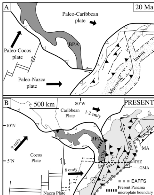
Fig. 2. Schematic tectonic reconstructions of northwestern South America and adjacent plates (A) at 20 Ma and (B) at present time (compiled and modified from Kellogg and Vega (1995), Taboada et al. (2000), and Trenkamp et al. (2001)). COc: Cordillera Occidental; CC: Cordillera Central; CO: Cordillera Oriental; MA: Mérida Andes; BPA: Baudo–Panama island arc (dark shaded area); SMBf: Santa Marta–Bucaramanga fault; GMA: Guatèque–Medina area. See discussion section for explanation about: TSZ: Transform shear zone (i.e. southern limit of the Caribbean plate); Bf: Bocono fault; EAFFS: East Andean frontal fault system. Northwestern Andes are in light grey.
