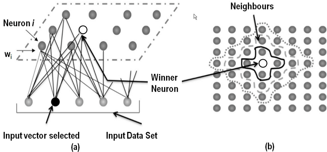
Figure 2 SOFM training algorithm
