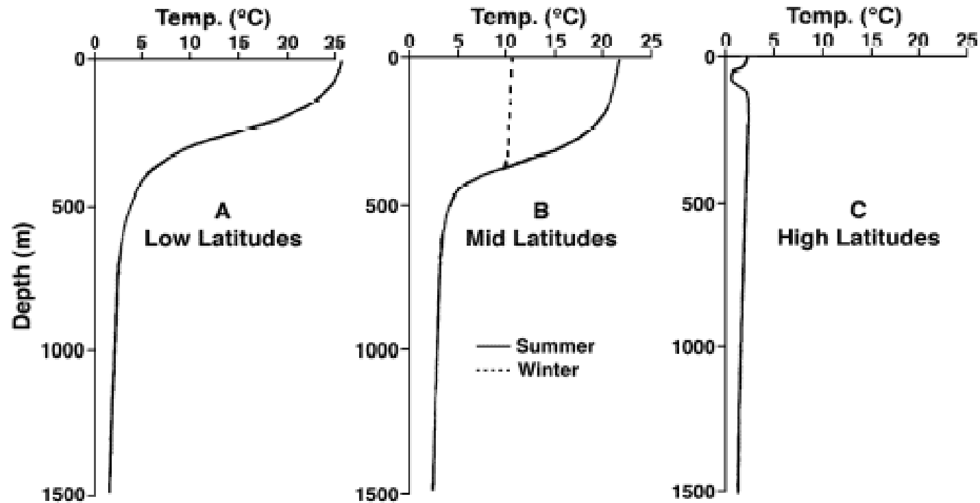
Typical Temperature Profiles
