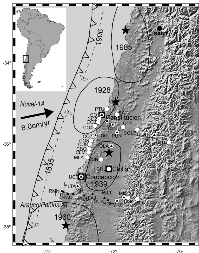
Fig. 1. Location of stations of the South Central Chile GPS experiment with respect to the seismotectonics context: open circles show location of GPS stations implanted in December 1996 and black triangles in March 1999. All stations were remeasured in April 2002. Black stars show the epicentres of the 1928, 1939, 1960 and 1985 earthquakes and large ellipses delimit the corresponding rupture zones. Dashed lines show the approximate extension of 1835 and 1906 earthquake ruptures. Plate convergence is from Nuvel-1A model (DeMets et al., 1994). Inset shows the location of the studied area in South America.
