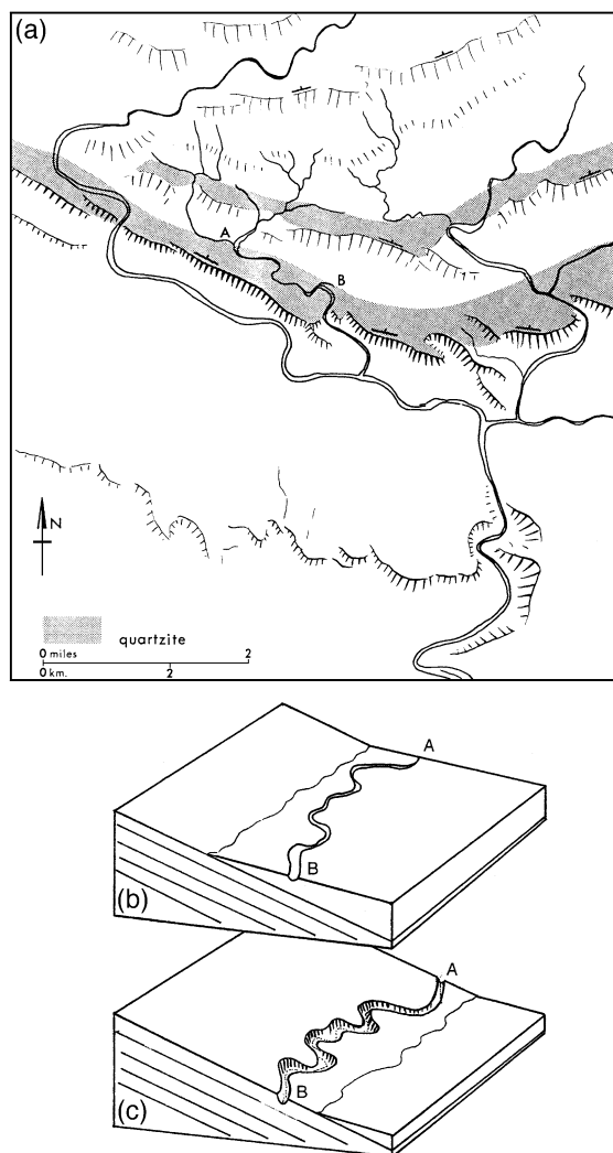
Fig. 31. (a) Plan of in-and-out gorges in the dip slope of a quartzite ridge near Arkaroola, northern Flinders Ranges. (b and c) The gorges, here seen from the north, are explicable in terms of valley impression in a dipping sedimentary sequence.
