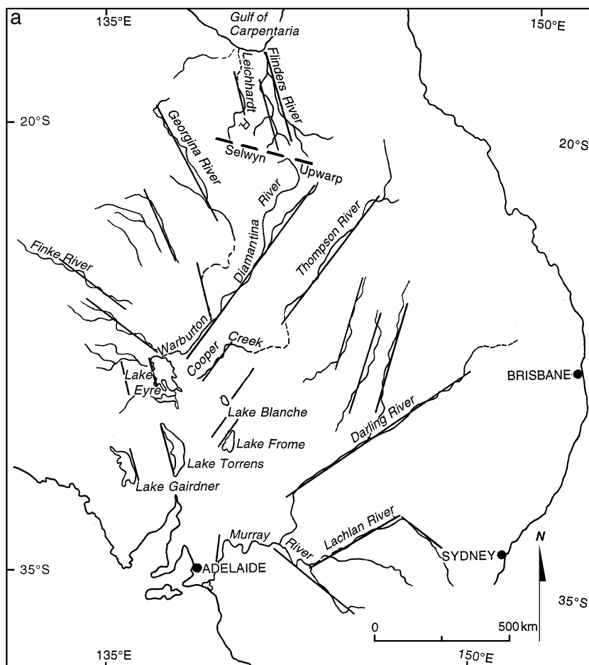
Fig. 19. (a) Underprinted straight rivers of central and northern Australia. Diversion of headwaters of the Diamantina River by the Selwyn Upwarps is also shown. Straight lines indicate lineaments. (b) Angular valley patterns developed along suggested underprinted fractures on the River Murray between Renmark and Morgan, South Australia. Downstream from A, river flows in gorge. Morgan Fault shown by heavy dashed line. The linked sector A–B is some 16 km long.
