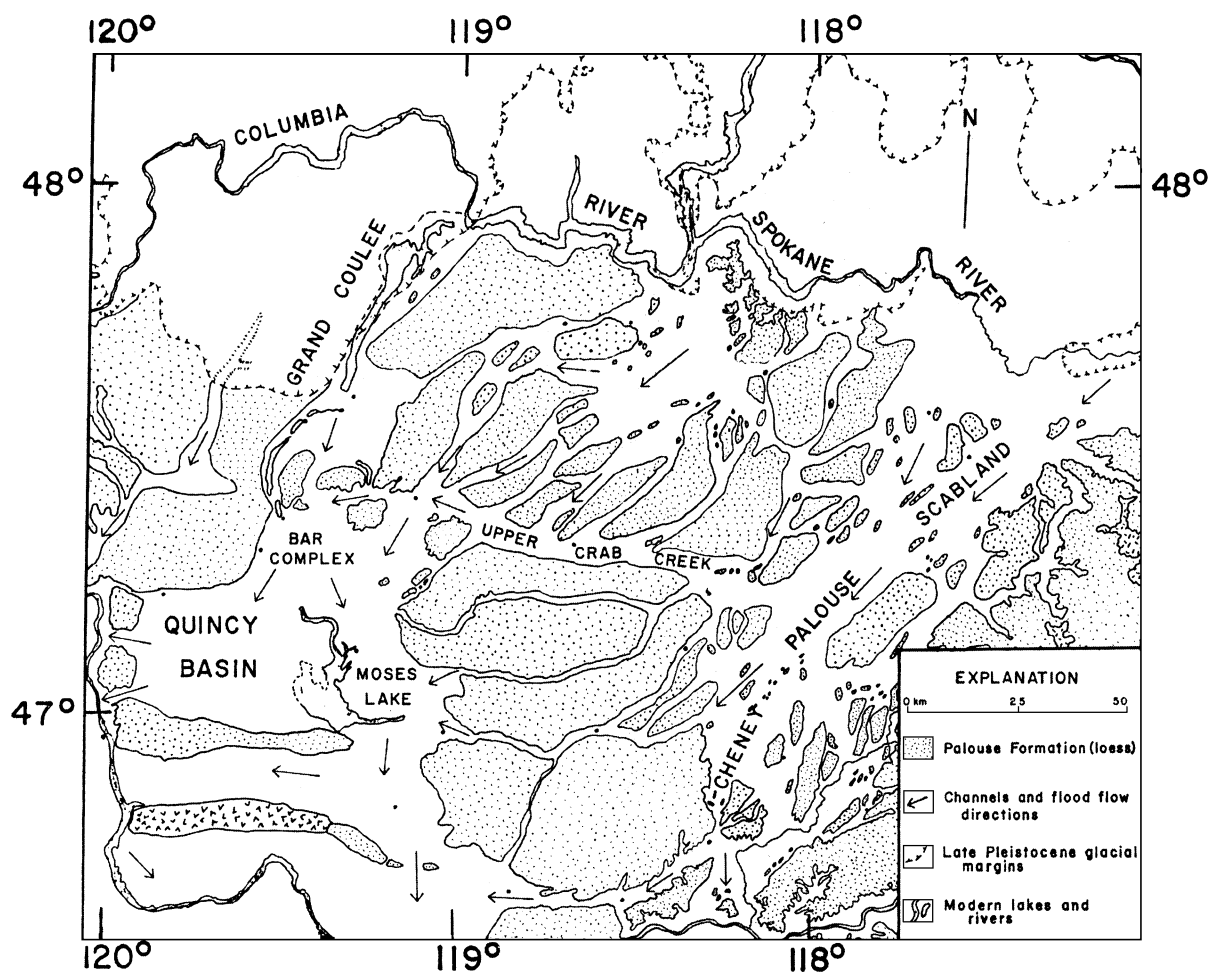
Fig. 39. The Channeled Scabland of northwestern USA showing the huge palaeochannels formed during the brief flood that followed the failure of a glacier dam that impounded Lake Missoula (after Baker, 1973).
