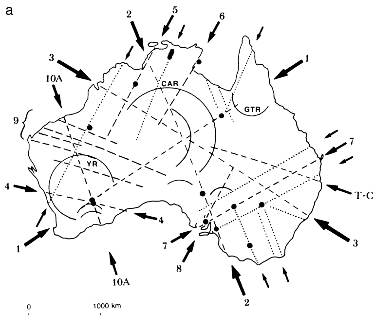
Fig. 24. (a) Numbered lineament corridors, and ring structures that have been exploited by streams, Australia (after O'Driscoll and Campbell, 1997). Black circles—major ore bodies, CAR—Central Australian Ring, GTR—Georgetown Ring, YR—Yilgarn Ring. (b) Disrupted and dismembered drainage of the Yilgarn Craton, Western Australia, with some lineament control (L) and also arcuate river remnants (A) linked to ring structures (after Van de Graaff et al., 1977).
