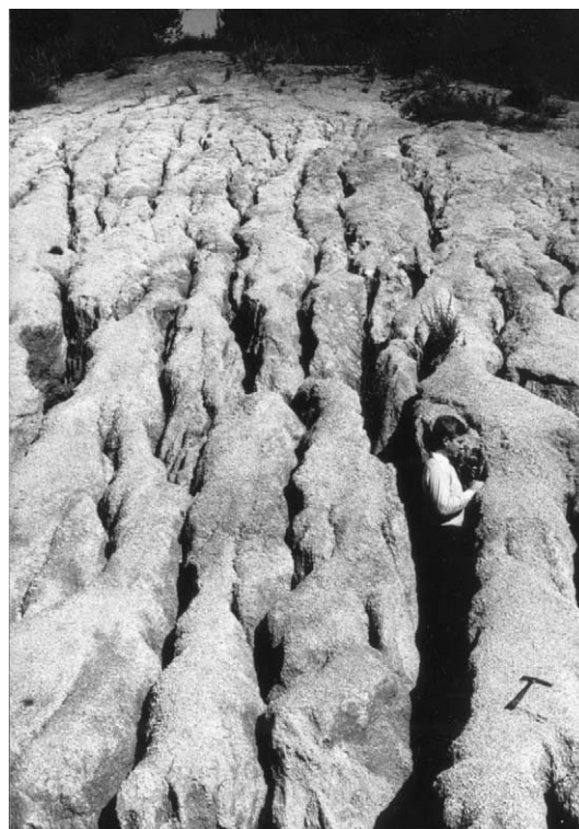
Fig. 11. Deep parallel–subparallel gullies in grus, near Paarl, Western Cape Province, South Africa.
