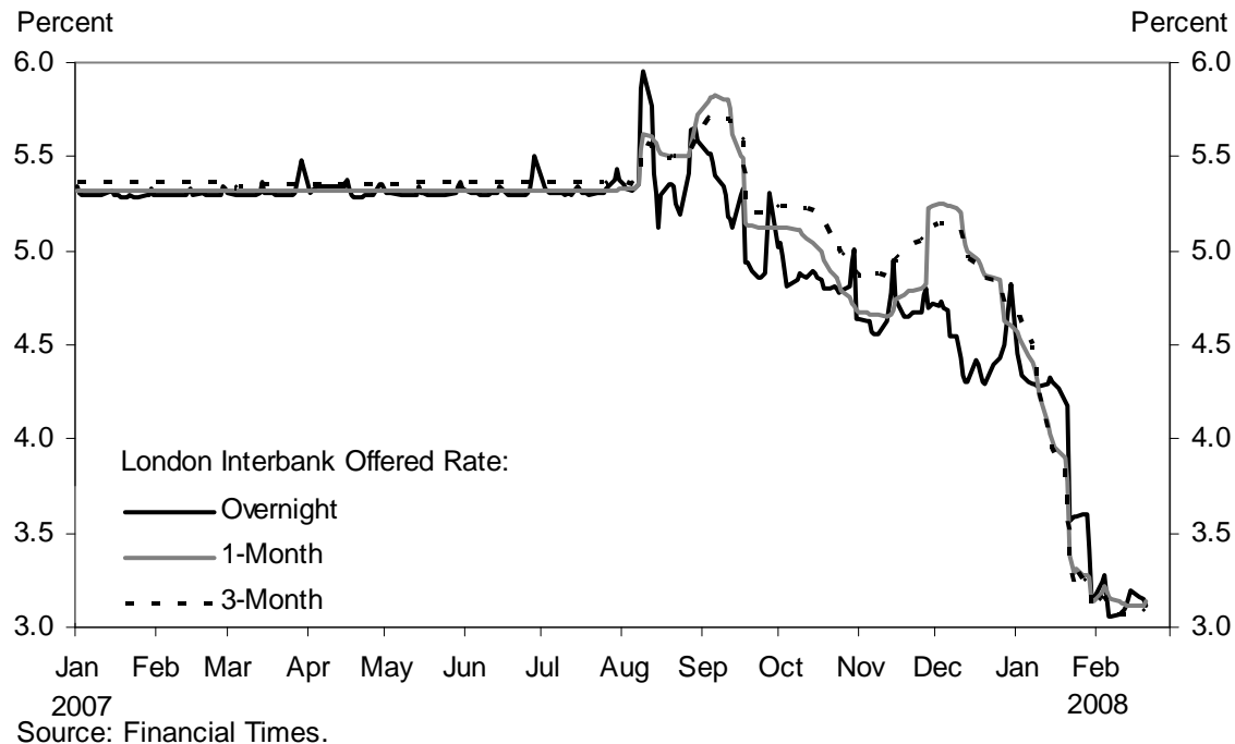
Exhibit 2.1 LIBOR Rate
