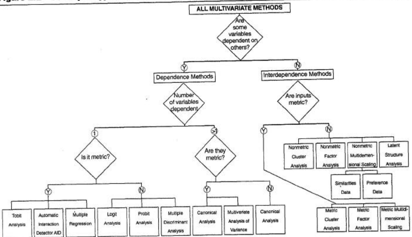
Figure 2.2 Principal Types of Multivariate Statistical Techniques
