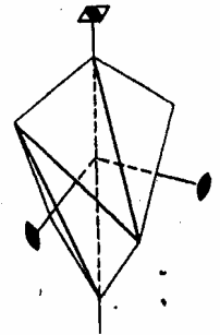
(29) Tetragonal scalenohedron (rhombic scalenohedron)
