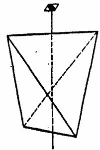
(33) Tetragonal disphenoid (tetragonal tetrahedron)
