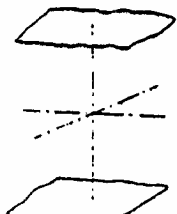
(2) Pinacoid (parallelhedron)
