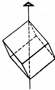
(31) Rhombohedron
