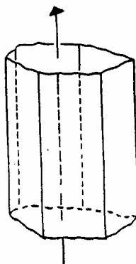
(7) Ditrigonal prism
