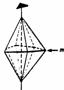
(21) Ditrigonal dipyrmaid
