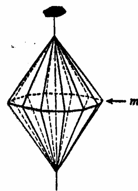
(25) Dihexagonal dipyrmaid
