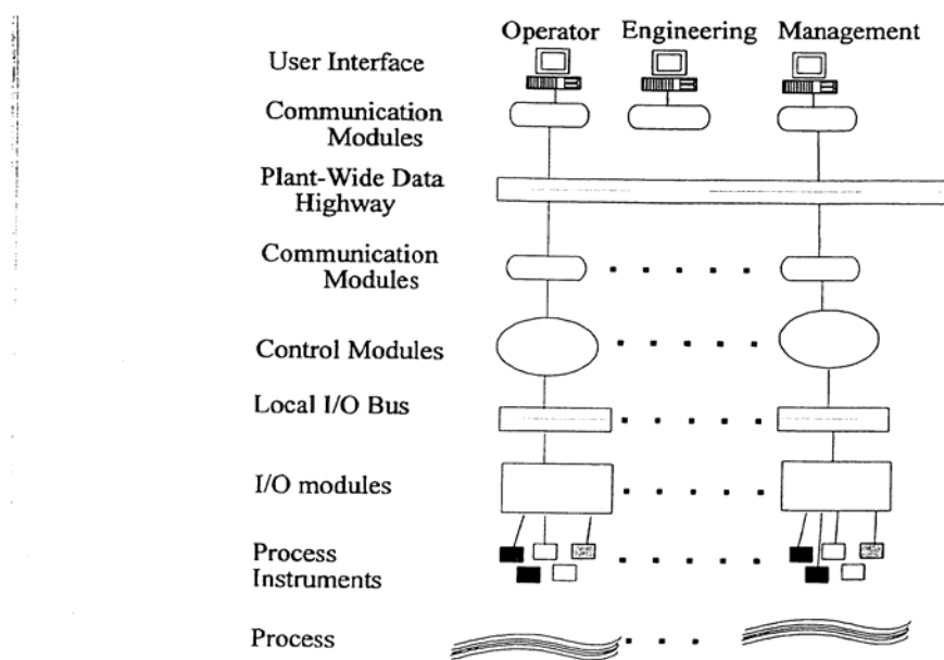
Fig. 2.4 A typical DCS configuration based on functional decomposition
