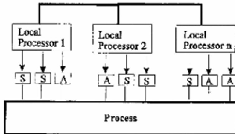
Fig. 2.2 Horizontally distributed system architecture
