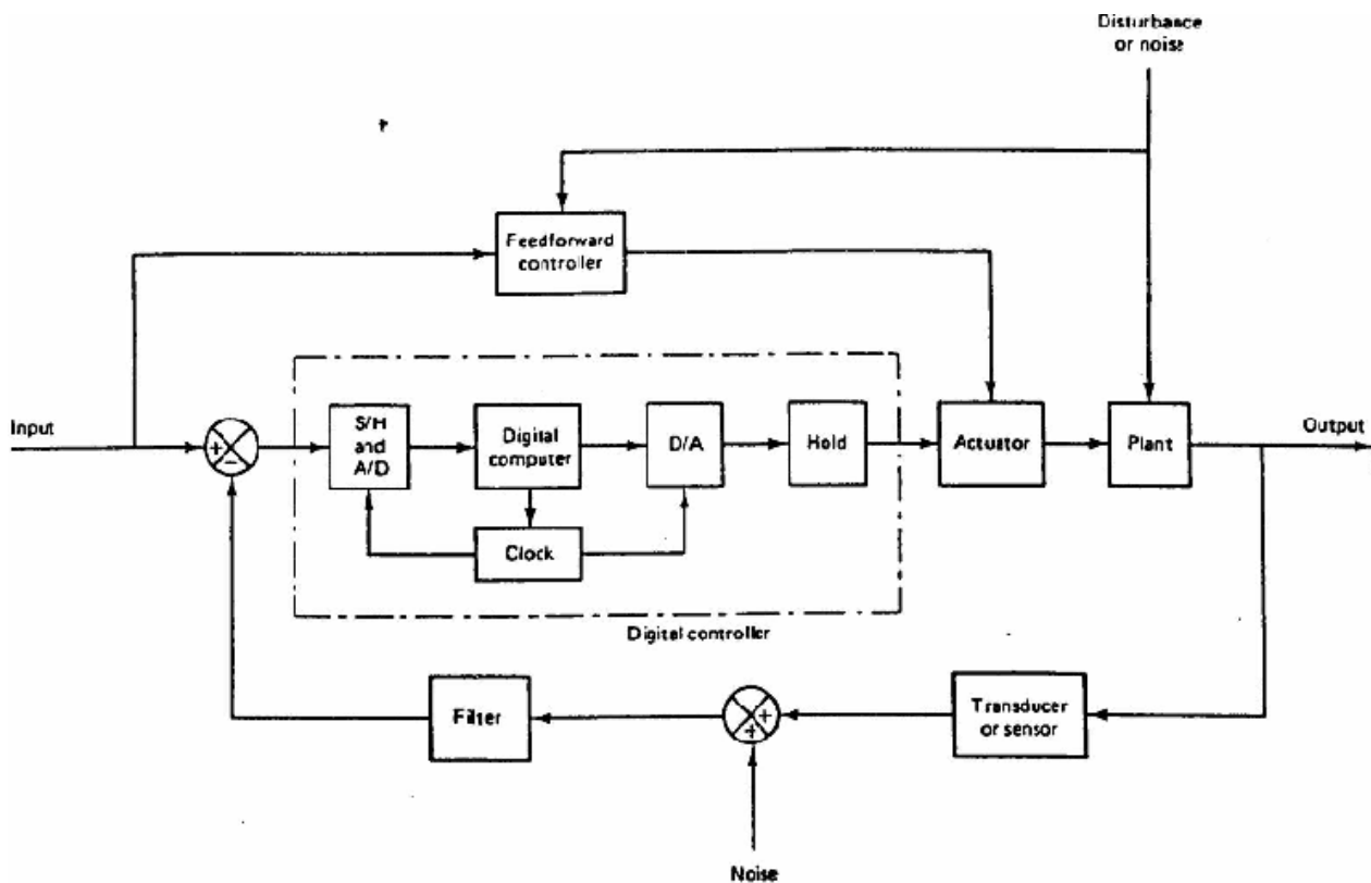
Figure 1-2 Block diagram of a digital control system.
