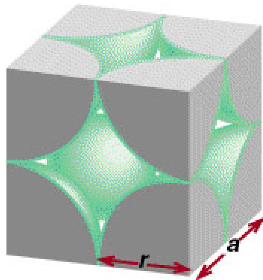
scc
