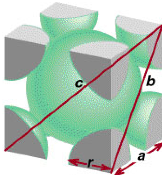
bcc
