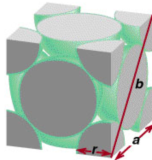
fcc
