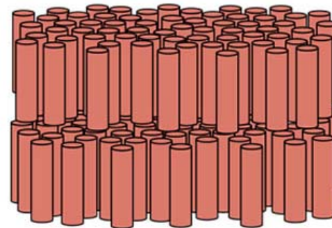
Smectic
