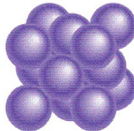
Face-centered cubic
