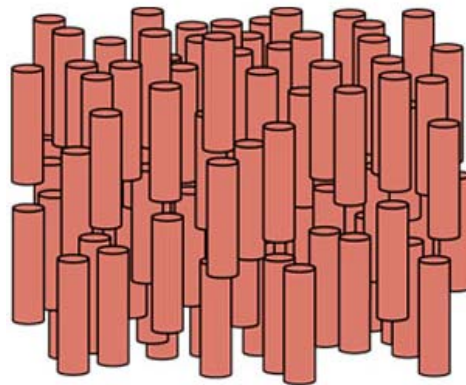
Nematic
