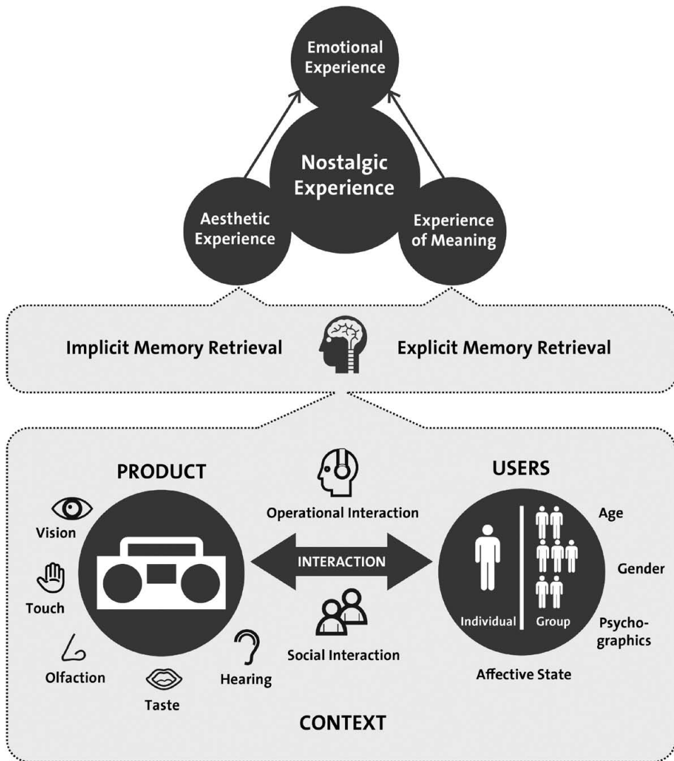
Figure 16. A heuristic model explaining the underlying process of DENE
