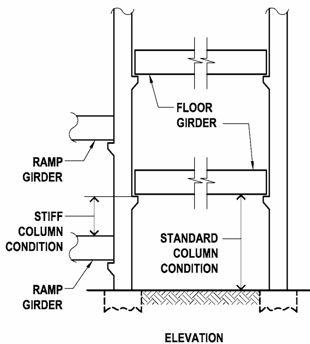
Figure 17.4.3-3: Accidental Reduction of Column Height at Ramp
