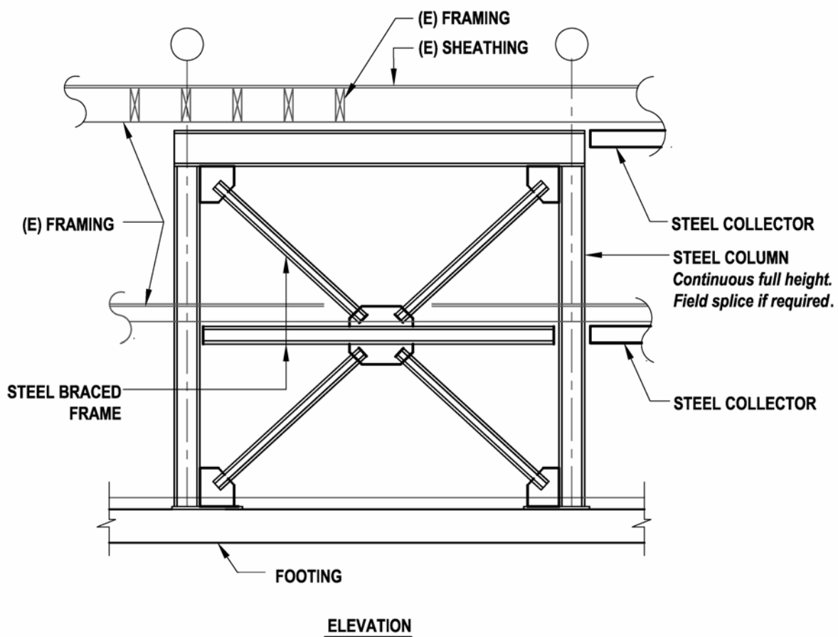
Figure 7.4.1-2: Two-Story Steel Braced Frame in a W2 Building
