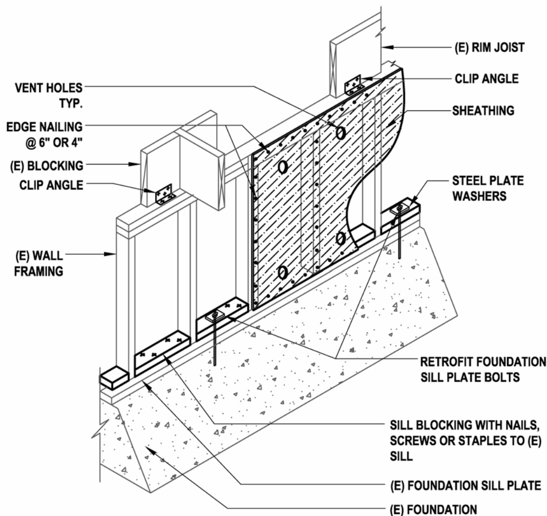
Figure 5.4.4-1: Cripple Wall Enhancement
