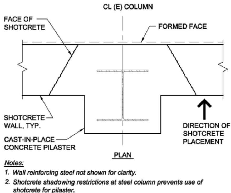
Figure 8.4.2-5: Combined Shotcrete and Cast-In-Place Construction
