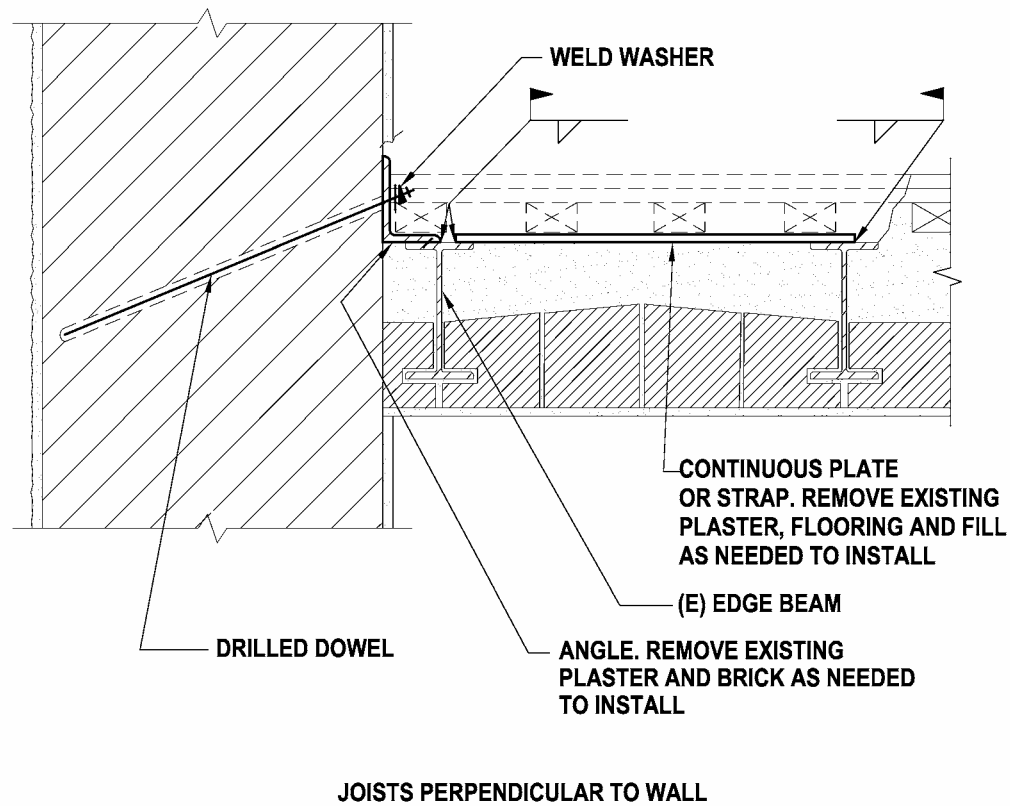
Figure 22.2.8-3: Add Wall-to-Diaphragm Ties and Chord for Masonry Flat Arch Floor - Access from Above the Floor
