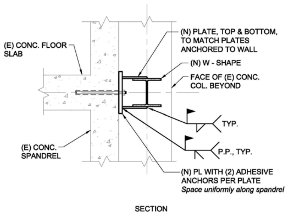
Figure 12.4.1-5: Braced Frame to Slab Connection
