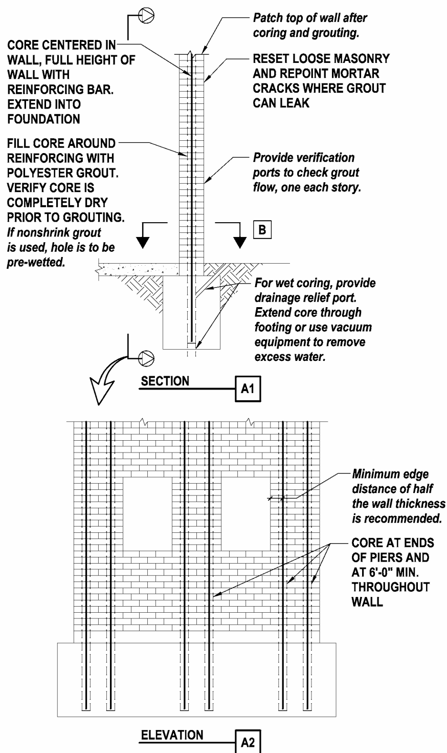
Figure 21.4.4-1A: Reinforced Cores
