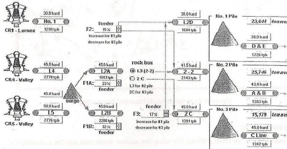
Figure 3: Primary Crusher/Conveyor Flowsheet
