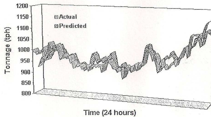
Figure 7: Example of Throughput/Feed Size Predictions
