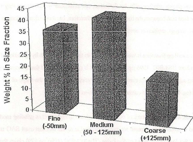
Figure 6: Typical Mill Feed Size Distribution
