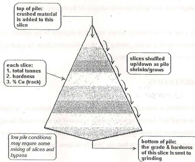
Figure 4: Schematic of Stockpile Model
