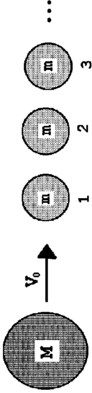
Fig. 1. A body of mass M , speed V_0 , undergoes a one-dimensional collision with an array of identical molecules of mass m at rest, with m < M . The momentum lost by the body as it moves forward is exchanged among the molecules away from the body in an orderly manner, without backscattering.
