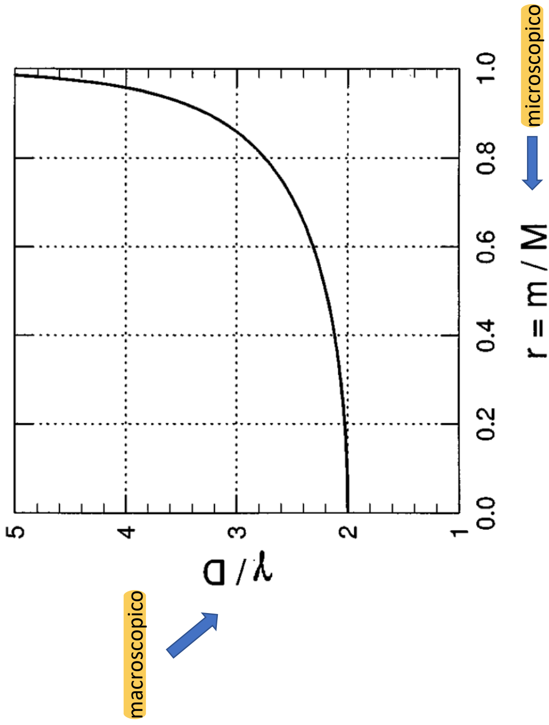
Fig. 3. Resistive coefficient \gamma as a function of molecule/body mass ratio.
