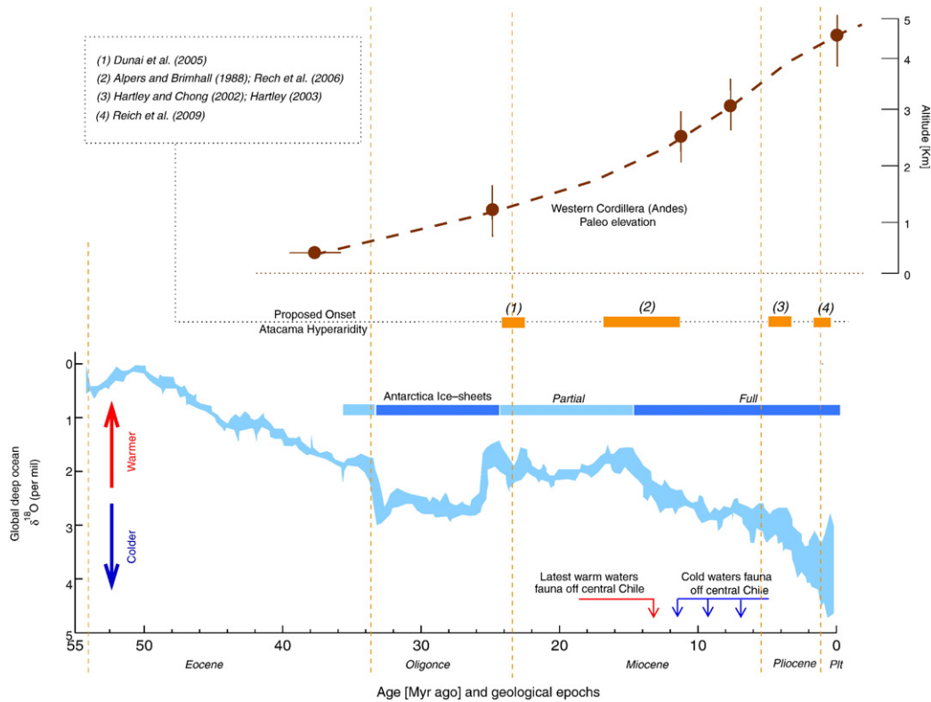
Fig. 2. Schematic chronology of the Andes cordillera paleoelevation (from Garzone et al., 2008; Farías et al., 2005; Hartley, 2003), proposed onset of Atacama hyperaridity (different sources indicated in inset), presence of Antarctic ice sheets and global deep-sea oxygen and carbonate isotopes reflecting cooling of the deep ocean and changes in ice volume (adapted from Zachos et al., 2001), and some key biotic events off north-Central Chile (from Bianucci et al., 2006; Walsh and Suárez, 2005; Ibaraki, 1992).
