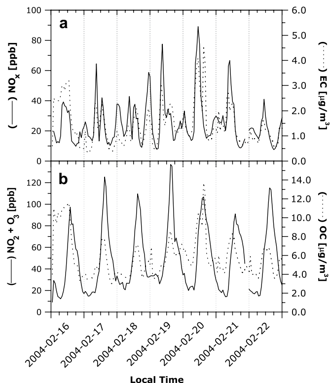
Fig. 4. Diurnal cycles of (a) \text{NO}_x (—) compared with EC (---) in \text{PM}_{2.5} and (b) \text{NO}_2 + \text{O}_3 (—) compared with OC (---) in \text{PM}_{2.5} at Las Condes (M label) station in seven representative days of February 2004. See Fig. 1 for station label.
