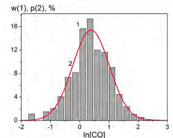
Fig. 7. The empirical distribution function w(1) of the carbon monoxide concentration in 2004 (Narodnogo Opolcheniya st.) and the log-normal approximated distribution p(2) .
