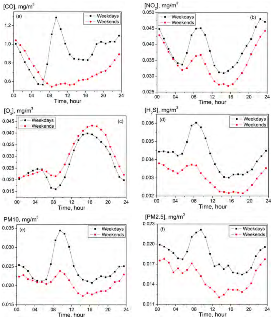
Fig. 4. Diurnal mean concentration cycles (2009) of (a) carbon monoxide (Balchug), (b) nitrogen dioxide (Mar'inskiy park), (c) ozone (Mar'inskiy park), (d) \text{H}_2\text{S} (Kosino), (e) PM10 (Shabolovka) and (f) PM2.5 (Kosino) at weekdays and at weekends.
