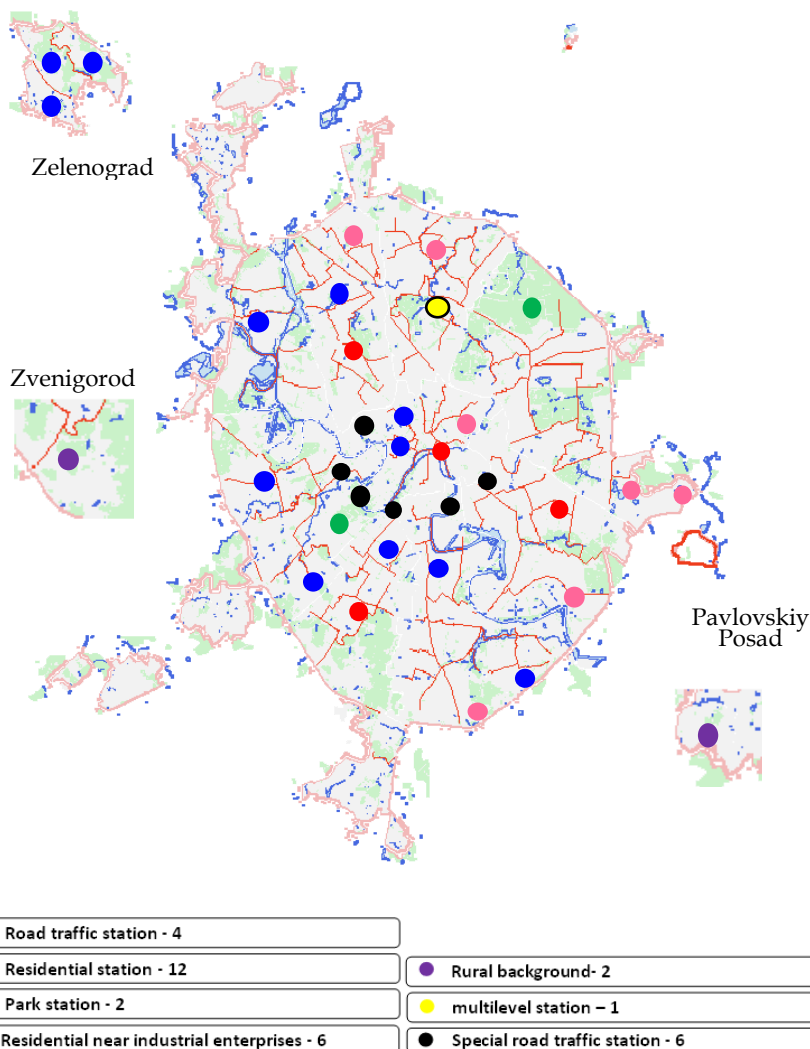
Fig. 1. Location of the automatic stations for the air quality monitoring in Moscow.
