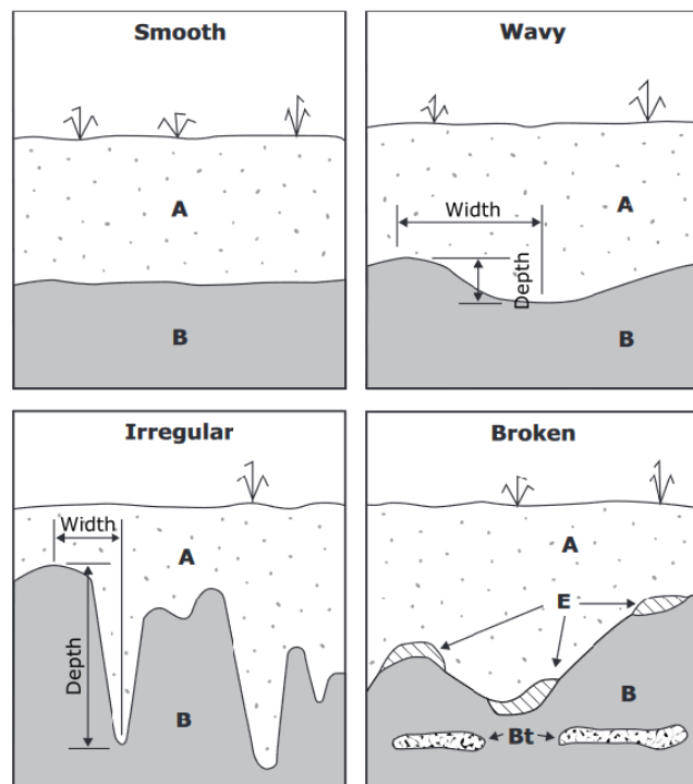
Figure 8.11: Shape of layer boundaries, Schoeneberger et al. (2012), 2-7, modified
