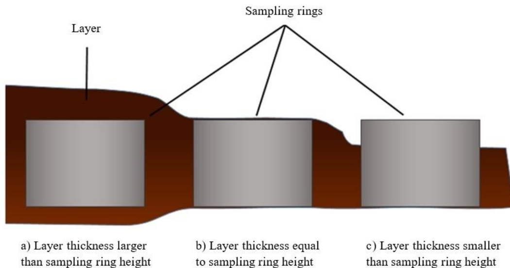
Figure 8.22: Volumetric sampling
