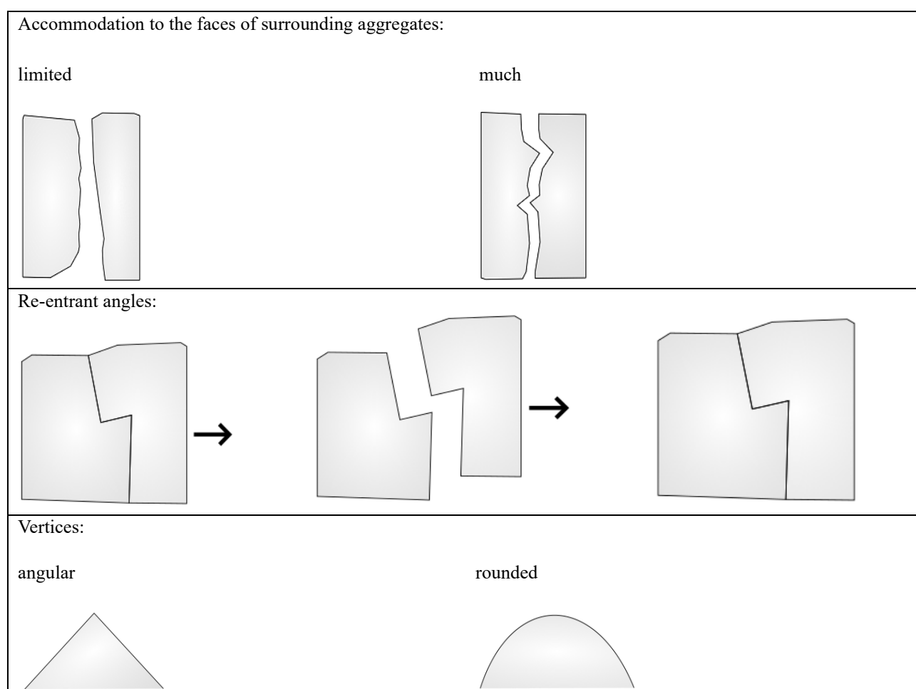
Figure 8.15: General terms of soil aggregate description
