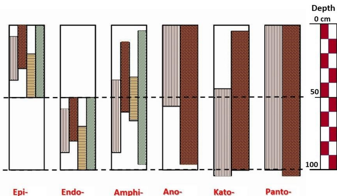
Figure 2.1: Specifiers to construct optional subqualifiers related to depth requirements and referring to a particular layer (Bathy- not illustrated), modified by S. Dondeyne
