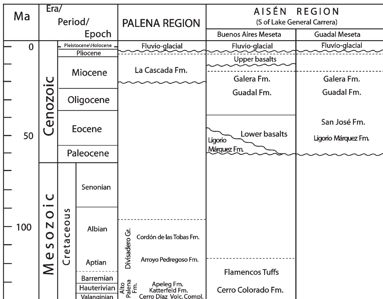
Fig. 3.69. Stratigraphic succession and correlation of Mesozoic and Cenozoic deposits in the Palena and Aisén (south of Lake General Carrera) regions. For the Aisén region, stratigraphic succession is given for the eastern region next to the borderline (Buenos Aires Meseta) and for the western region (Guadal Meseta) (corresponding with stratigraphic units of Fig. 3.65).
