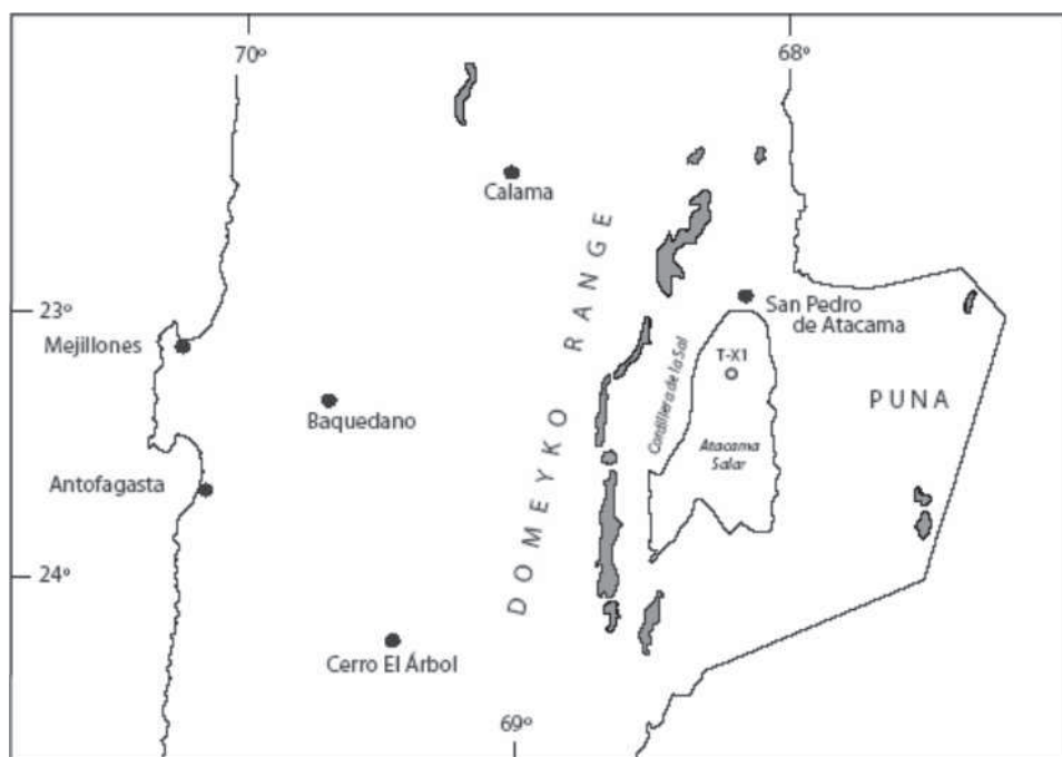
Fig. 3.33. Distribution of the foreland deposits of the second stage of Andean evolution in the Antofagasta–Salar de Atacama region with location of the Toconao–X1 hydrocarbon exploration well. Outcrops NW of Calama correspond to the Tolar Formation, an age equivalent of the deposits east of the Domeyko Range. The easternmost deposits in the Puna plateau close to the border correspond to small outcrops of the Late Cretaceous Argomedo–West Fissure Fault, the Argomedo–West Fissure (Falla Oeste) Fault developed along the Domeyko Range and its northern prolongation, the Sierra del Medio. The Calama Formation deposits
