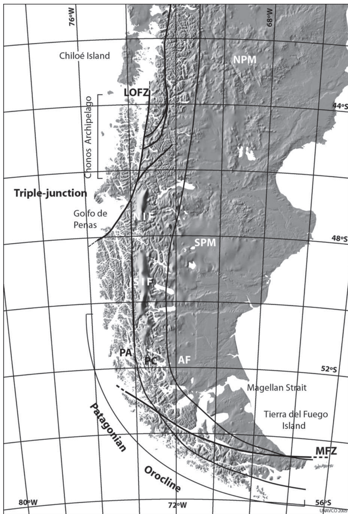
Fig. 3.64. Digital elevation model of the Chilean Andes south of 42°S with indication of the main geographic, tectonic and morphostructural features. Abbreviations: AF, Andean Foreland; LOFZ, Liqueñe-Ofqui Fault Zone; MFZ, Magallanes Fault Zone (main trace); NIF, northern ice-field; NPM, North-Patagonia Massif; PA, Patagonian Archipelago; PC, Patagonian Cordillera; SIF, southern ice-field; South Patagonia Massif.
