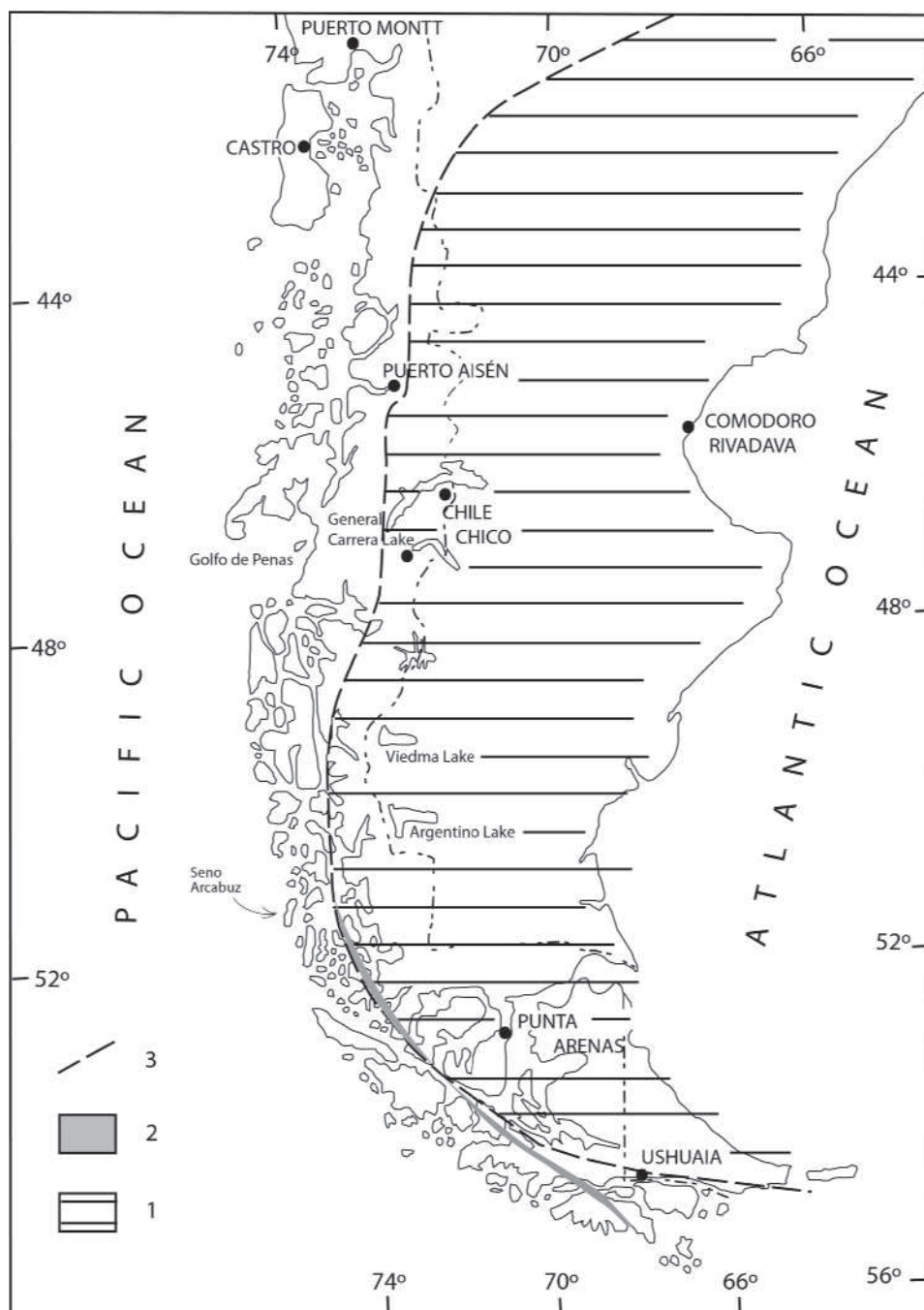
Fig. 3.66. Distribution of the deposits of the first stage of Patagonian evolution. Key: 1, Complejo Porfiritico de la Patagonia (Ibañez Group, Quemado Group, Tobifera Formation) or Chon Aike magmatic province (see Mpodozis & Kay 1990). 2, Ophiolitic suite of the 'Rocas Verdes Basin', south of 50°S. 3, Western limit of exposures. The Complejo Porfiritico de la Patagonia most probably reached the westernmost regions of present-day Patagonia. (See Seno Arcabuz Shear Zone, Hervé & Fanning 2002).
