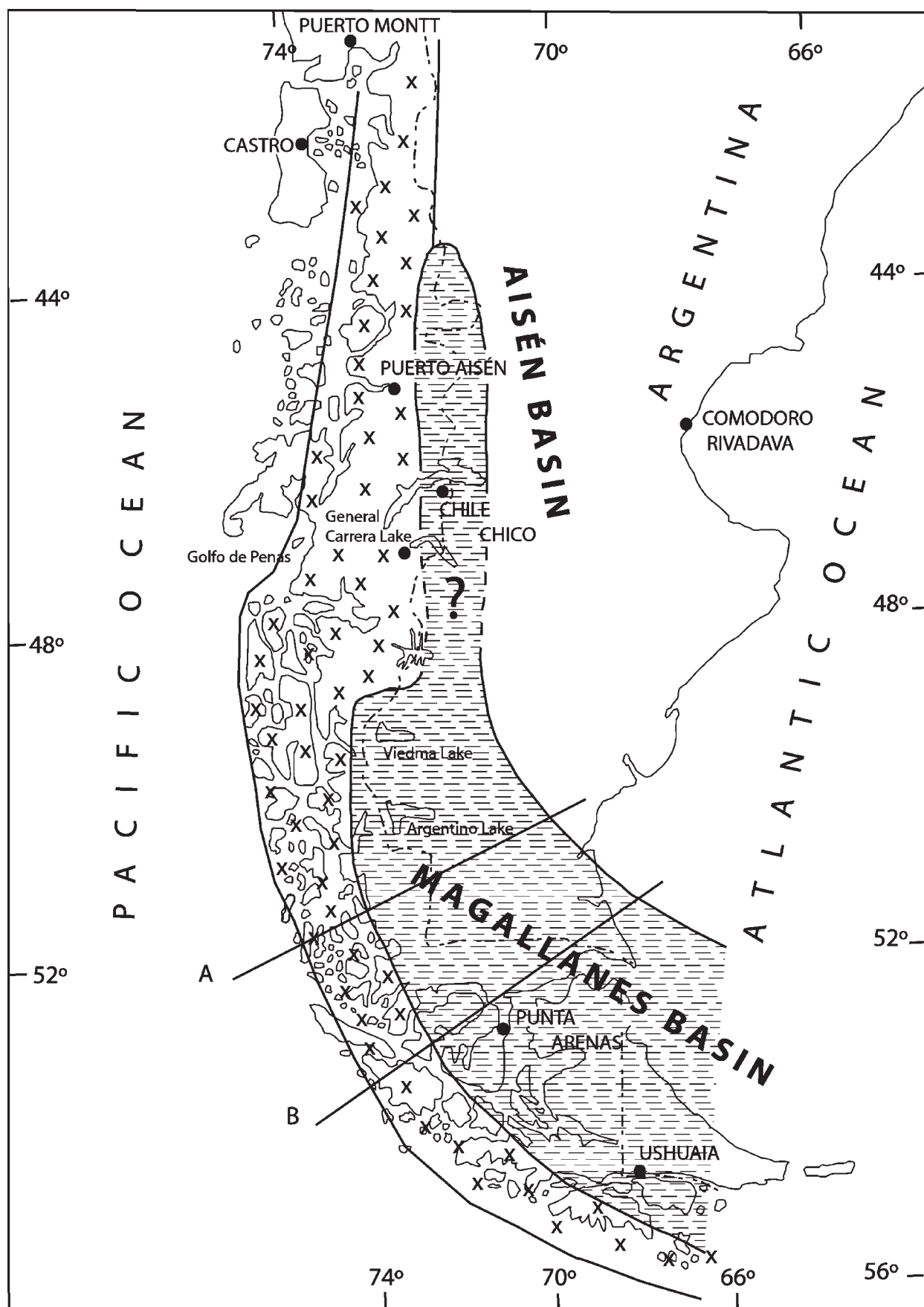
Fig. 3.67. Second stage of Andean evolution in Patagonia. Distribution of the Aisén and Magallanes basins and the Patagonian Batholith.
