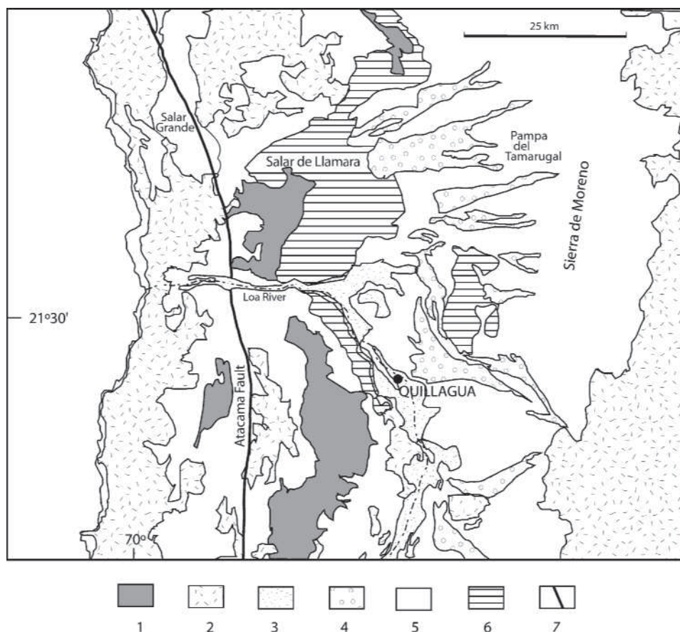
Fig. 3.47. Simplified geological map from the Quillagua region showing the relationship between the El Loa Formation (Quillagua lacustrine deposits), the Salar (evaporitic) deposits and the huge alluvial cones descending from the Sierra de Moreno. Salar development is controlled in this region by uplift of the Coastal Cordillera along the Atacama Fault Zone. Key: 1, El Toco Fm (Devonian); 2, Mesozoic units; 3, El Loa Formation; 4, Alluvial cones; 5, other Cenozoic deposits; 6, Salar de Llamara and other older salars (Soledad Formation of Skarmeta & Marinovic 1981); 7, trace of the Atacama Fault (highway runs along the fault trace).
