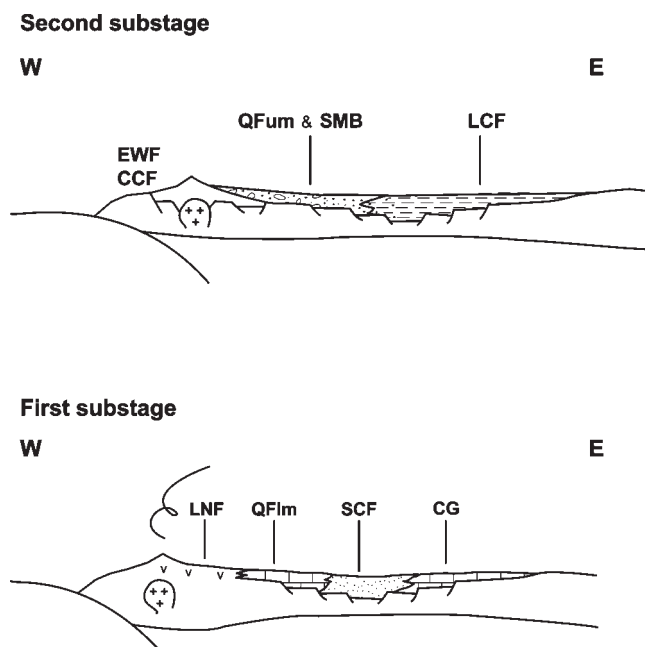
Fig. 3.20. Schematic palaeogeographic sections for the first and second substages of the first Andean stage in northernmost Chile, based on the region of Antofagasta. Note the forearc deposits in the second substage. Abbreviations for the first substage: LNF, la Negra Formation; QFIm, 'Quinchamale Formation', lower member; SCF, Sierra El Cobre Formation; CG, Caracoles Group. Abbreviations for the second substage: CCF, Caleta Coloso Formation; EWF, El Way Formation; QFum, 'Quinchamale Formation', upper member; SMB, San Manuel Beds; LCF, Llanura Colorada Formation.
