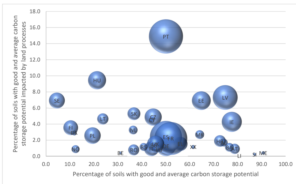
Figure 3.3 Comparison of percentage of soils with good and average carbon storage potential and percentage of soils with good and average carbon storage potential affected by all land processes (y-axis) (10)
