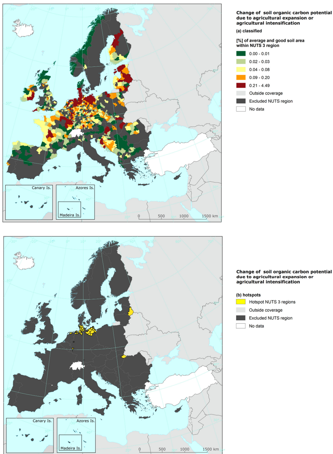
Map 4.4 Hotspots of soil organic carbon impairment due to agricultural intensification and expansion, classified map (a) and hotspots (b)
